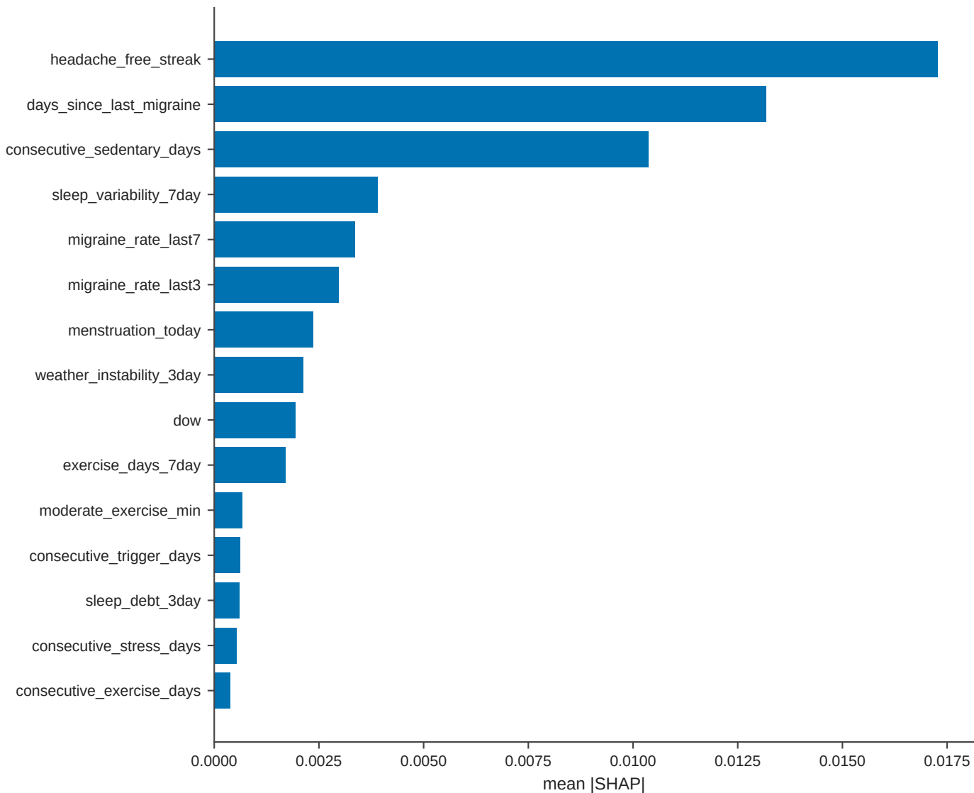
migraine headline (XGB-HP020 / full / chrono / 70-30) - feature attribution
