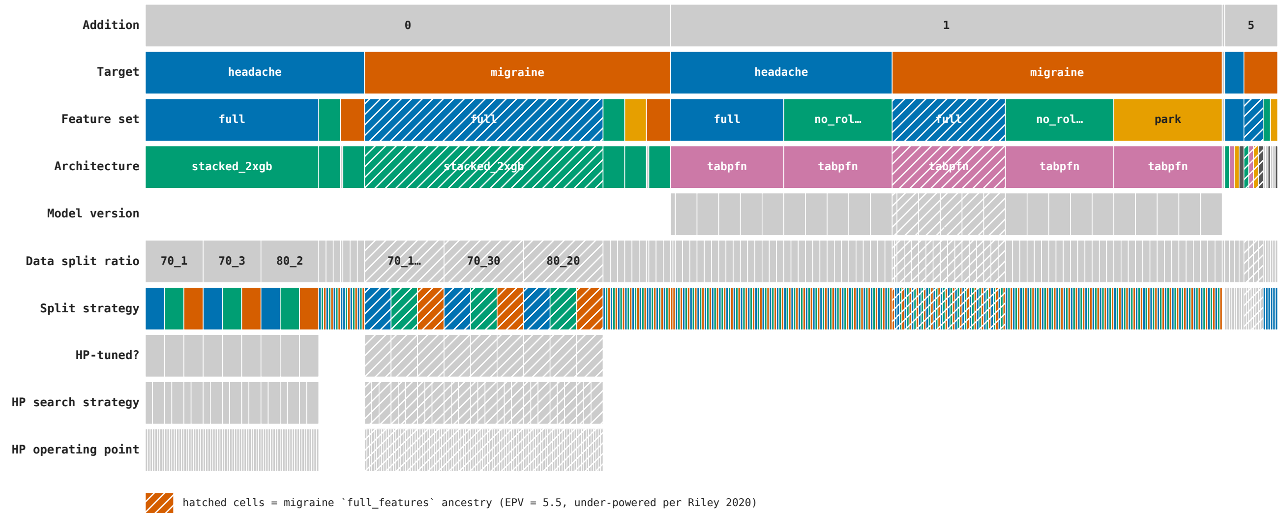
Discovered experiment leaves (470 total) - icicle plot
