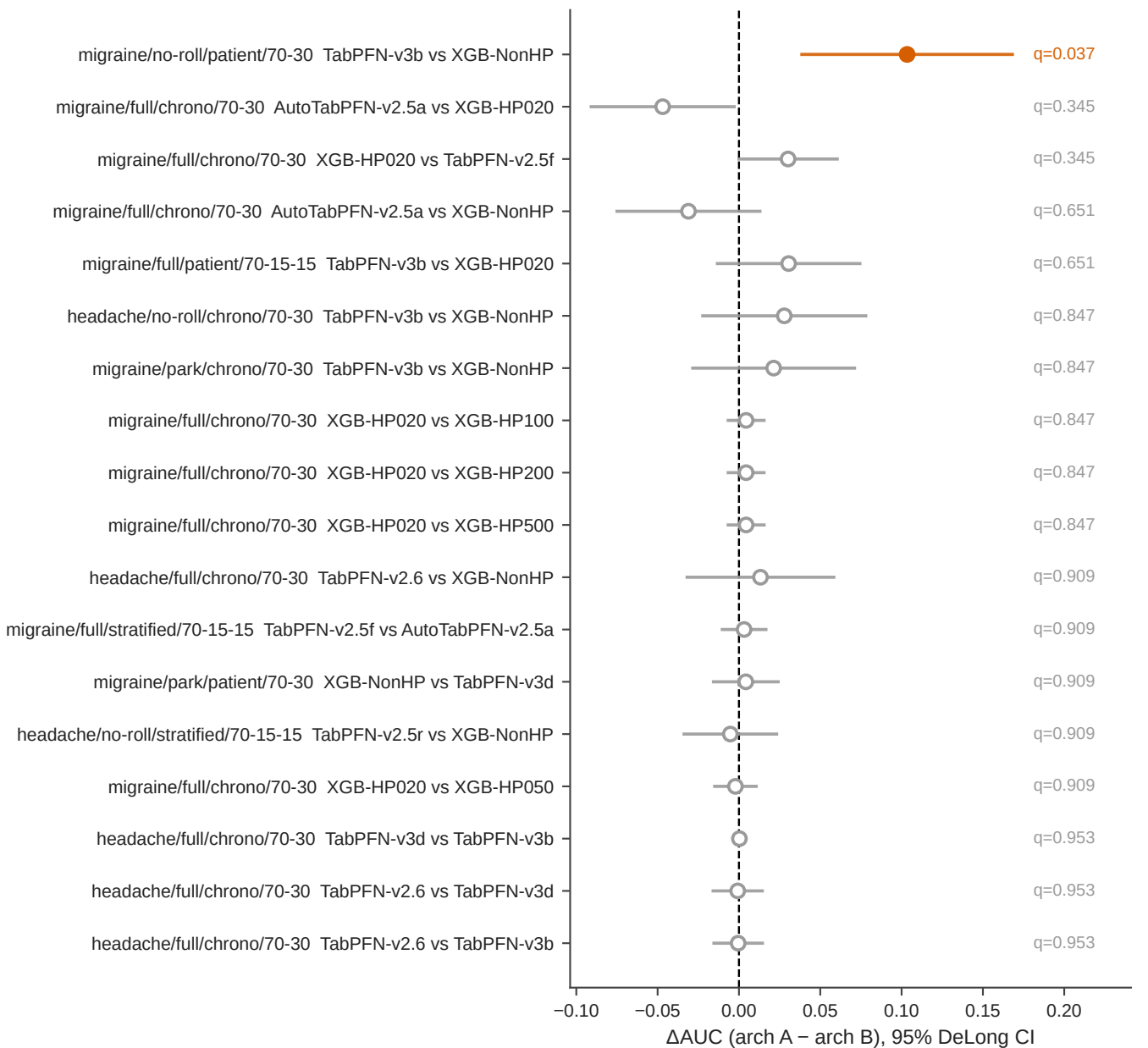
Paired DeLong + BH-FDR ( q \leq 0.05 ) across 18 cross-architecture tests; 1 significant after multiplicity correction
