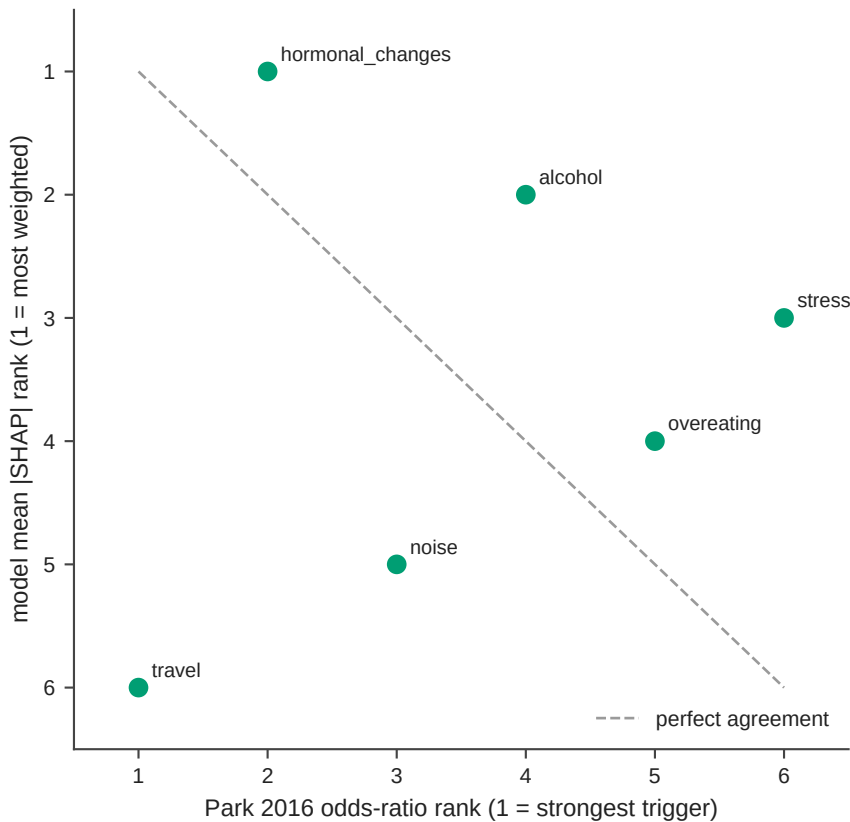
headline xgboost - Spearman rho = -0.26
