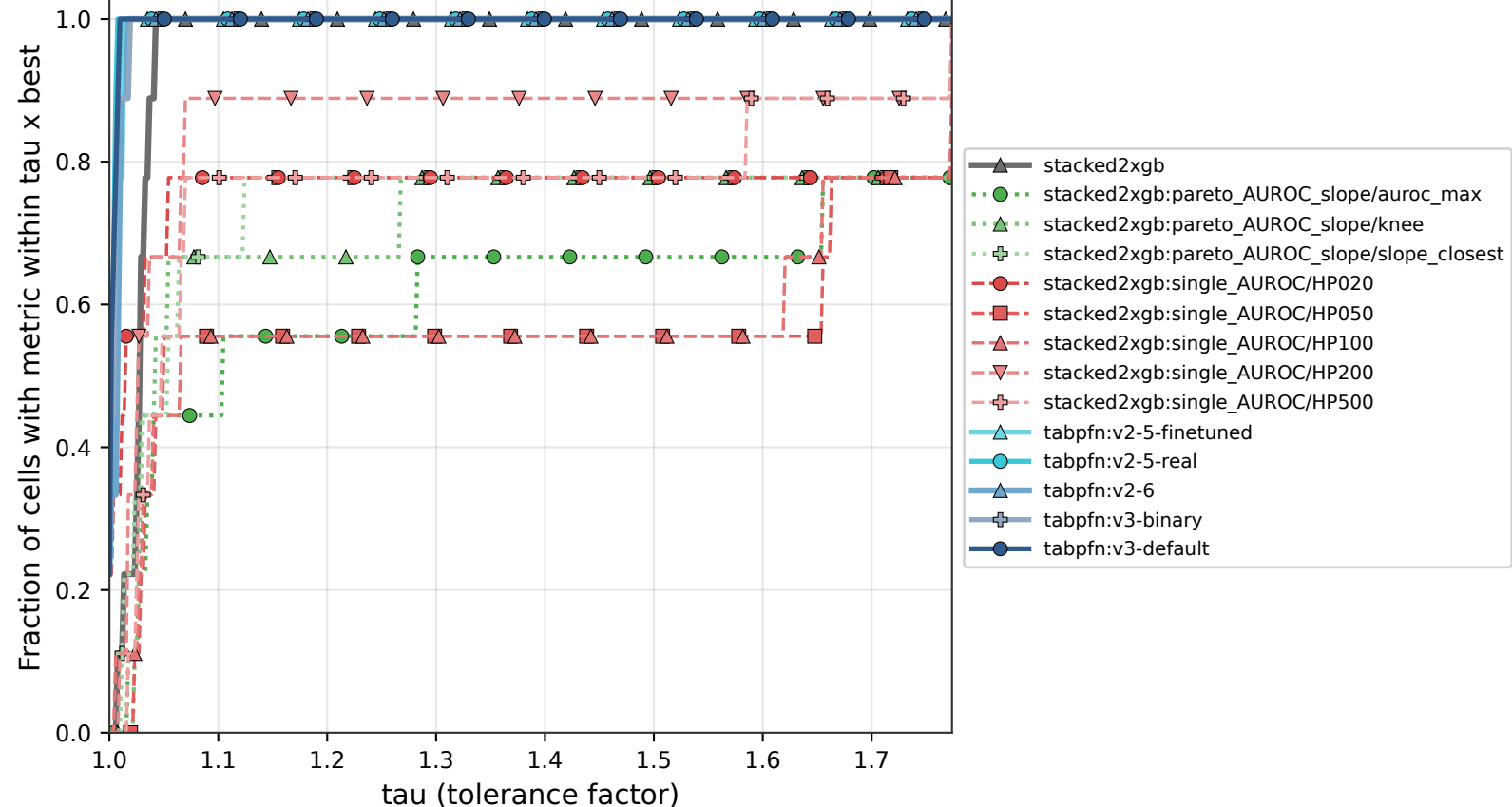
Performance profile (Dolan-More) - headache AUROC (n_cells = 9)
