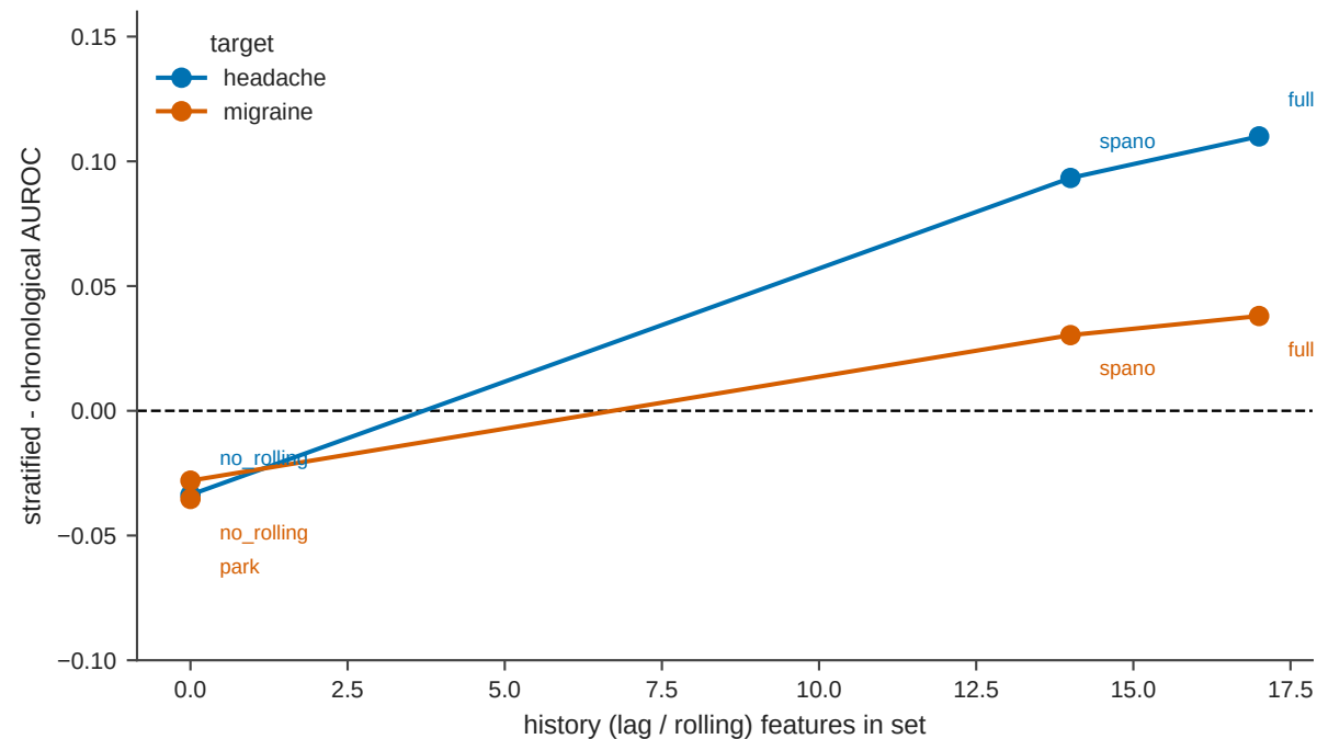
Stratified-split optimism scales with history features (XGB-NonHP held constant; mean over ratios 70/30 + 70/15/15)
