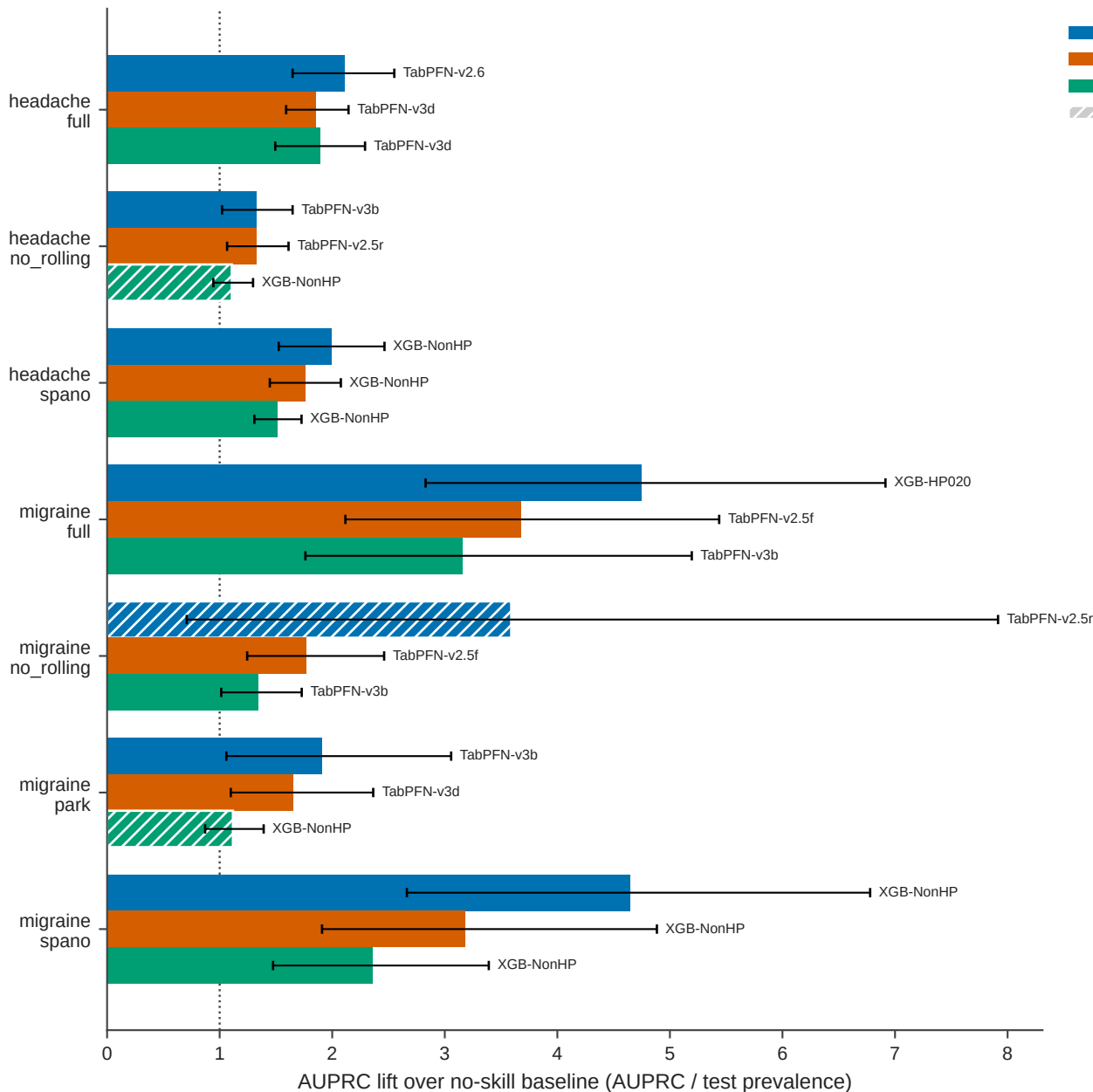
Precision-recall skill by split type, per cell (headline)
