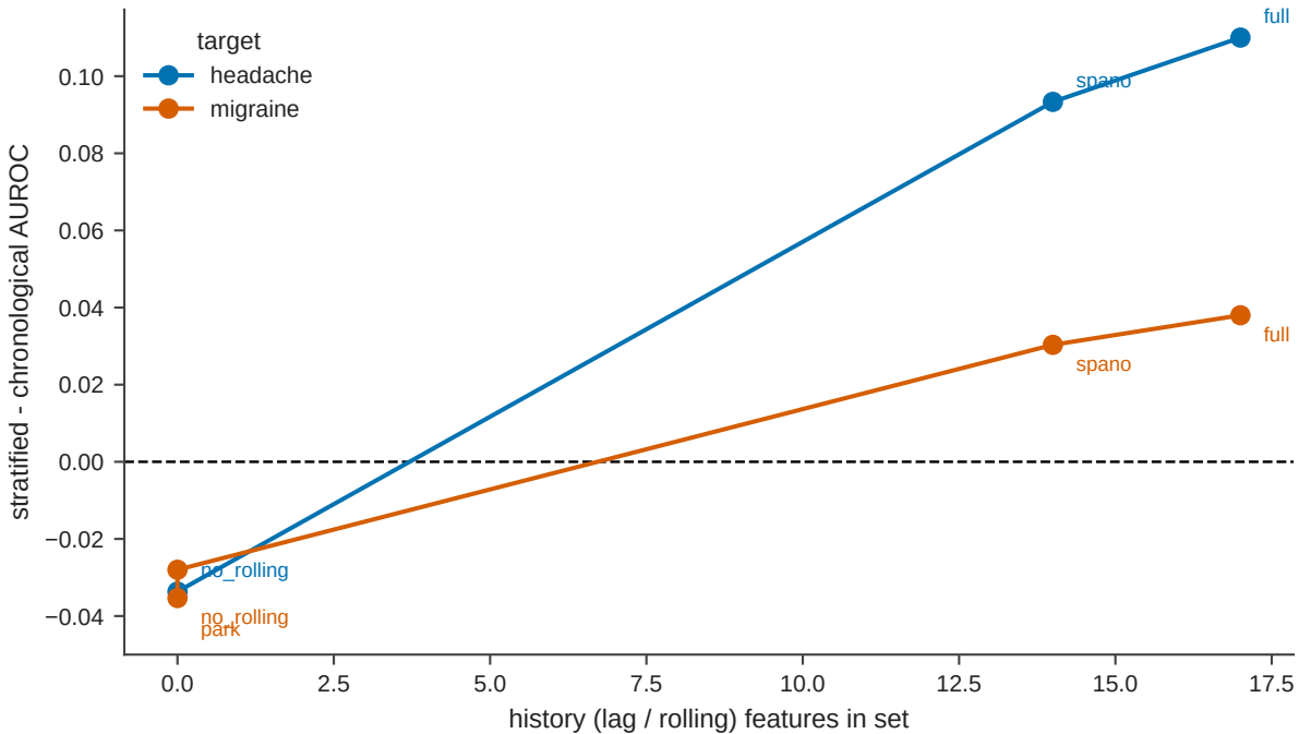
Stratified-split optimism scales with history features
