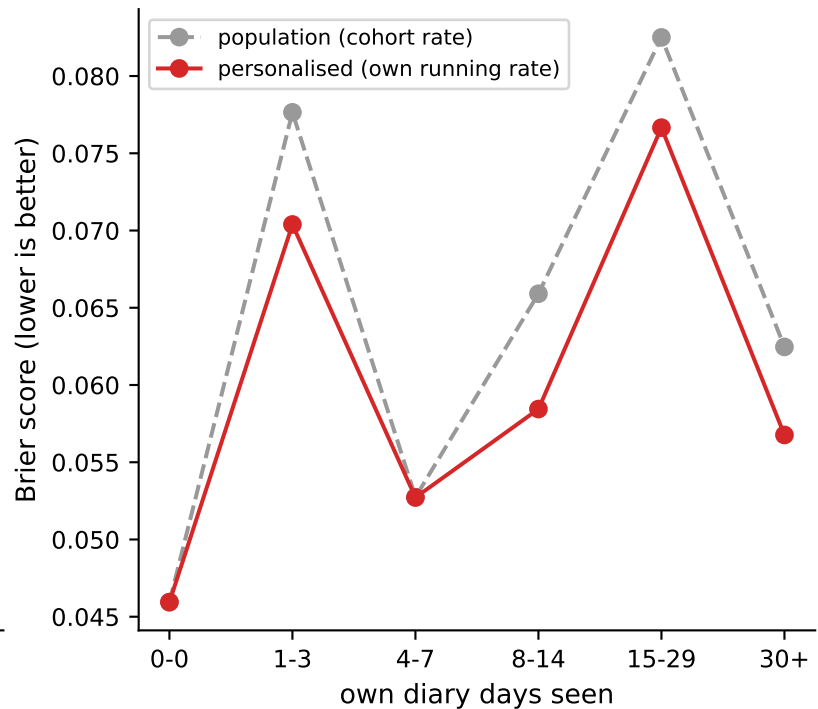
migraine (personalisation helps from ~1 own day)
