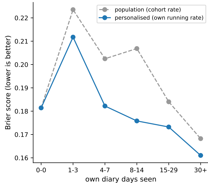
headache (personalisation helps from ~1 own day)
