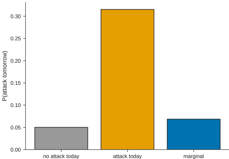
First-order transition - migraine (RR=6.3, p=8.8e-67)
