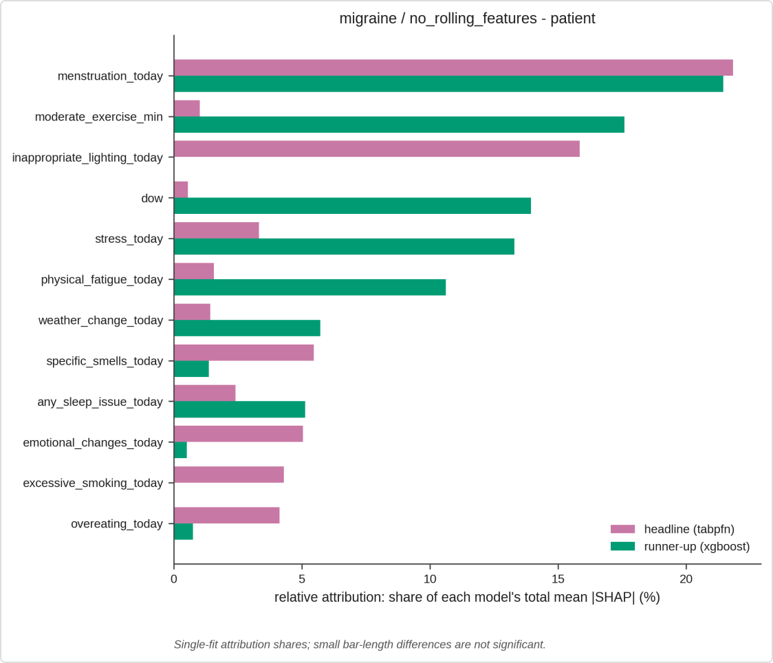
Cross-architecture attribution: each model's top features as a share of its own total mean |SHAP| (headline vs runner-up). Normalised because the two explainers' absolute magnitudes are not comparable; rank agreement is in the table above.
