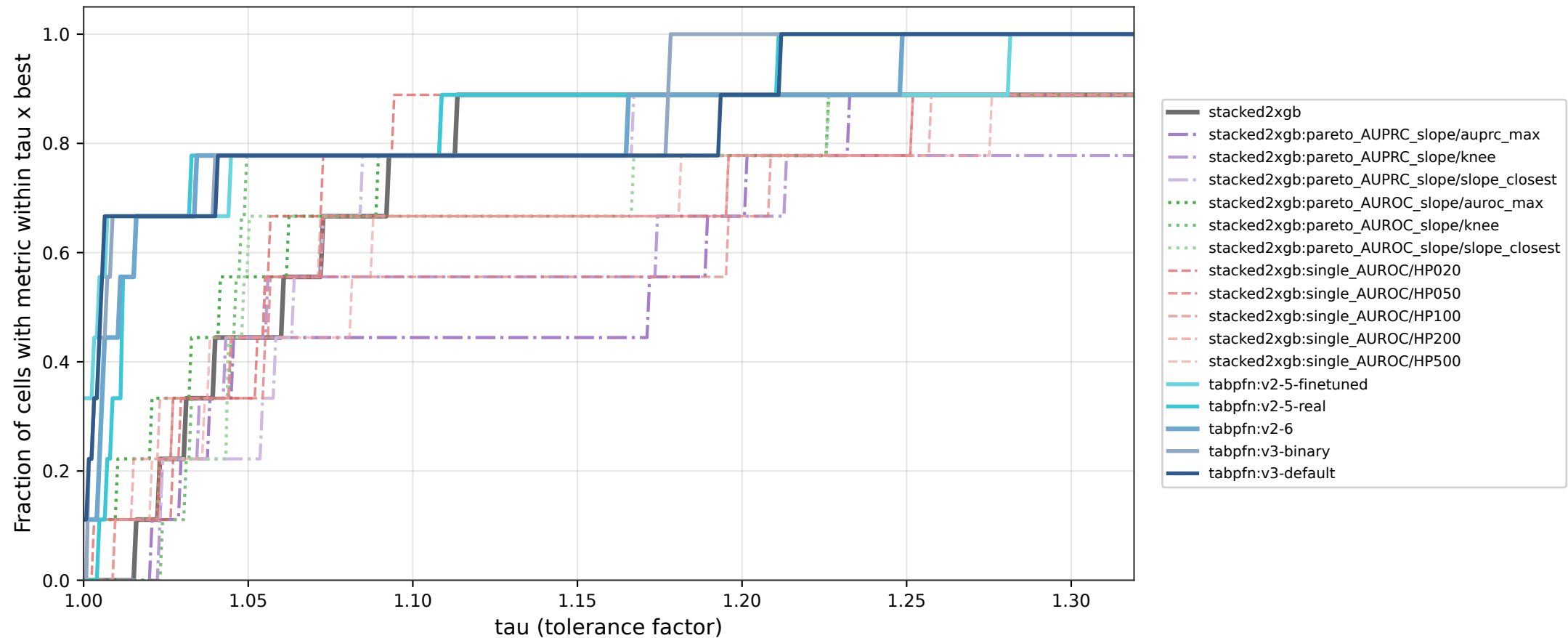
Performance profile (Dolan-More) - migraine AUROC (n_cells = 9)
