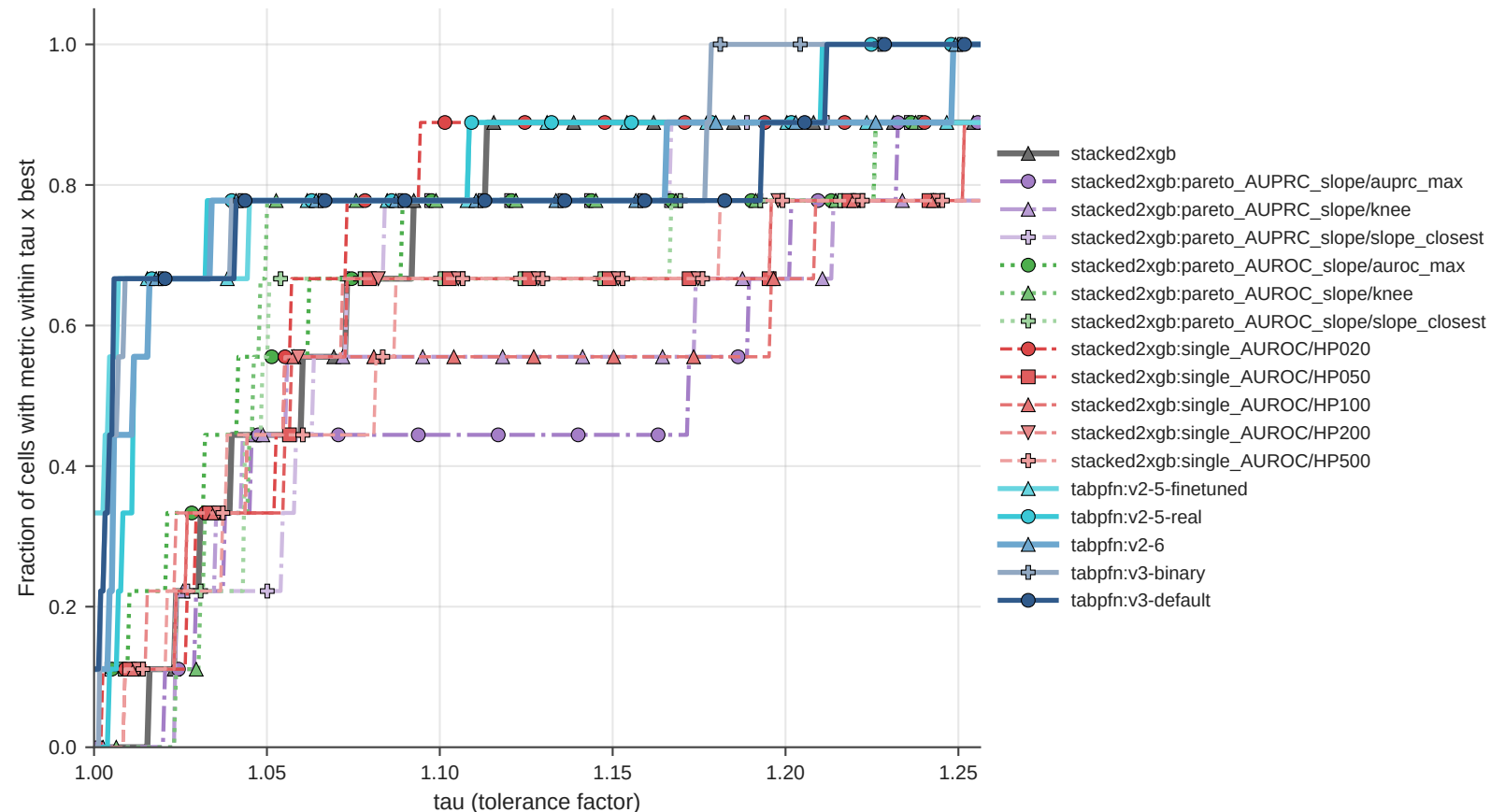
Performance profile (Dolan-More) - migraine AUROC (n_cells = 9)
