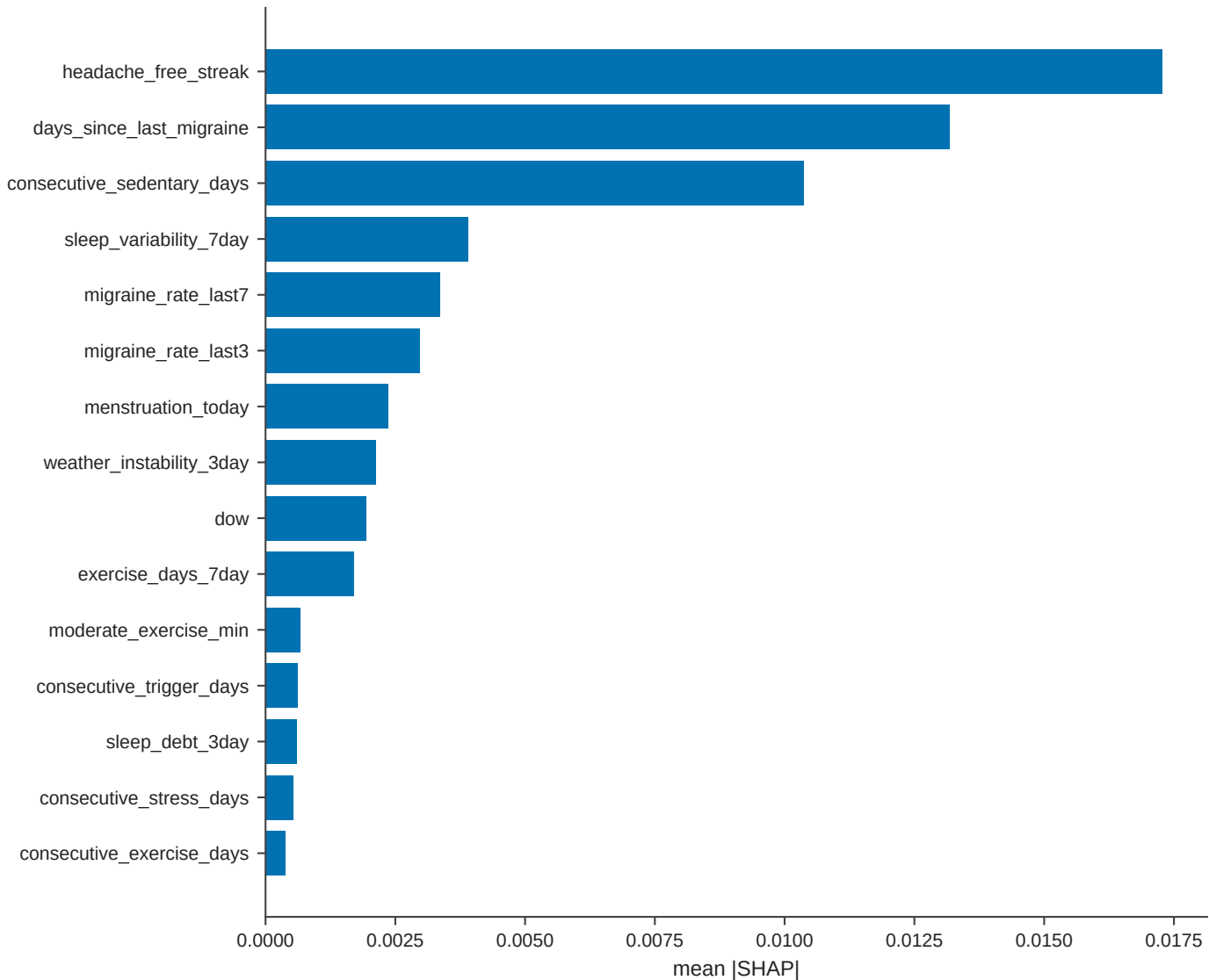
migraine headline (xgboost) - feature attribution
