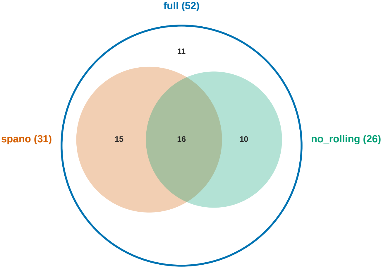
Feature-set structure - nested Euler (schematic)
