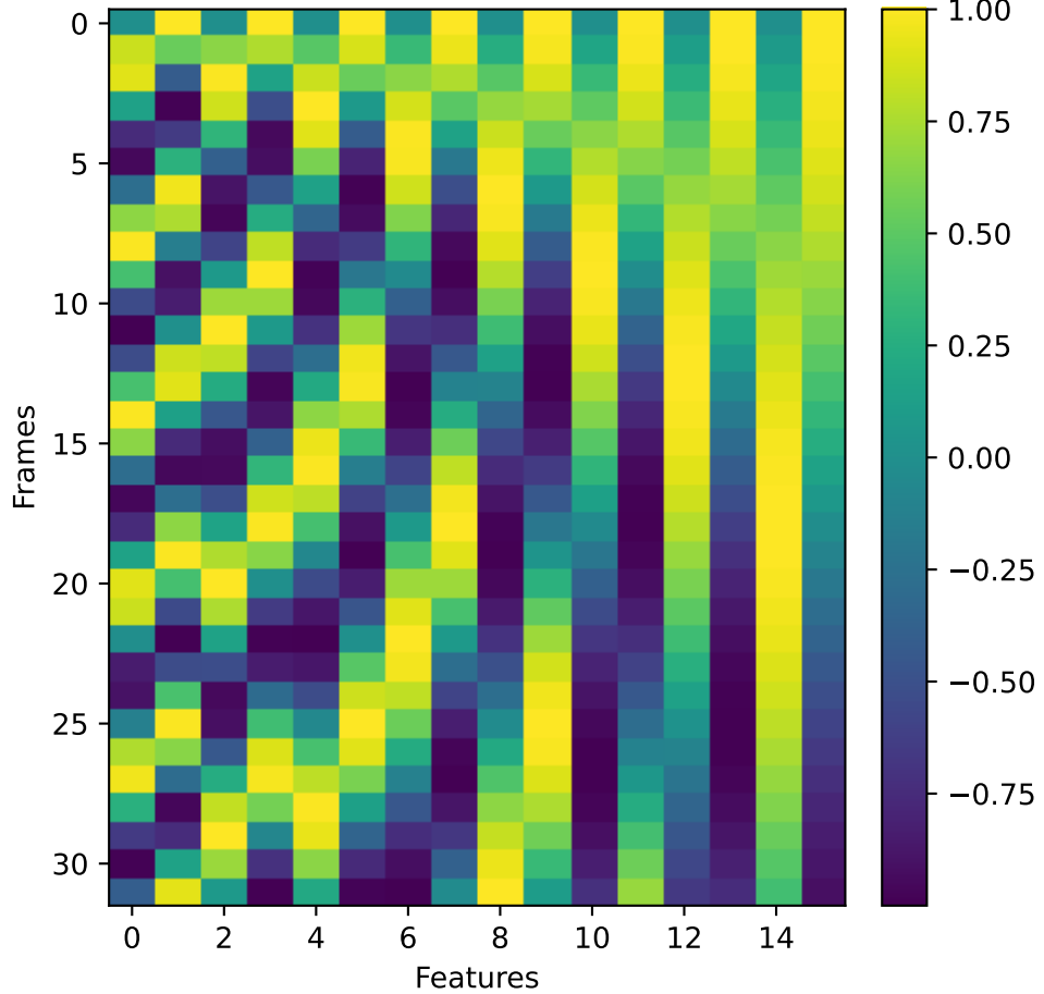
Modified positional encoding (base=16)
