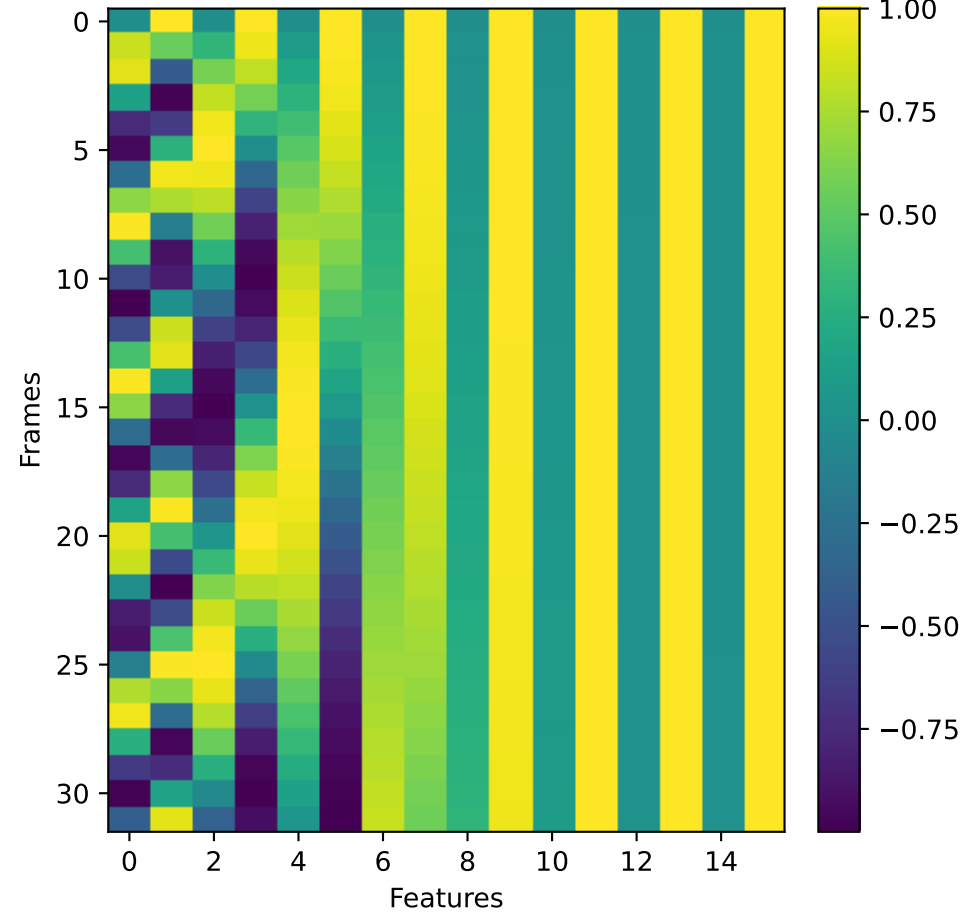
Original positional encoding (base=10000)
