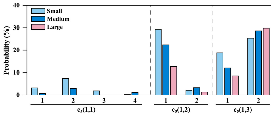
Fig. 11. Frequency distribution of flood control hazard forms.
