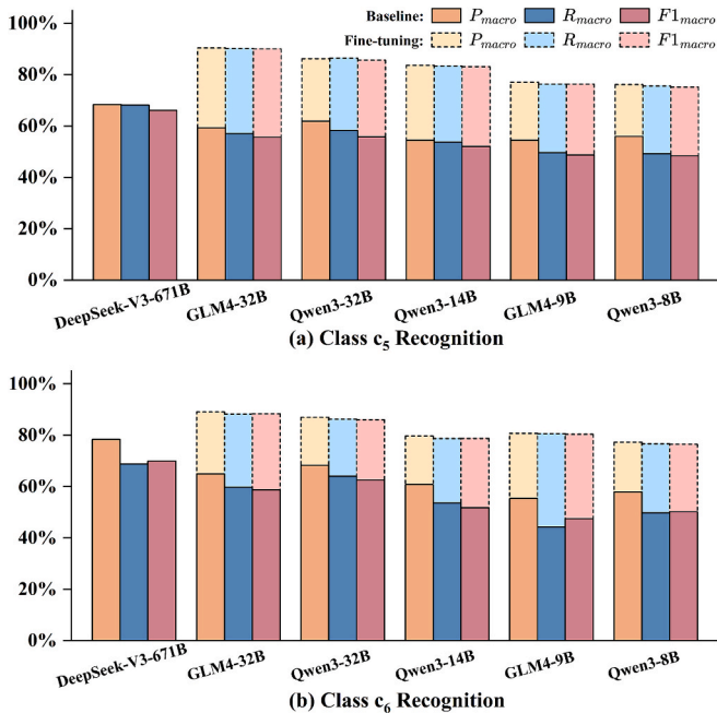
Fig. 6. Model performance before and after fine-tuning.
