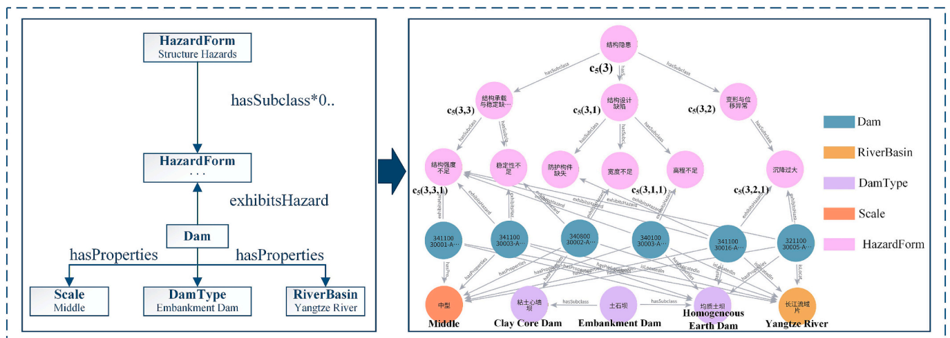
Fig. 9. Example of Structural Hidden Danger Knowledge Retrieval.
