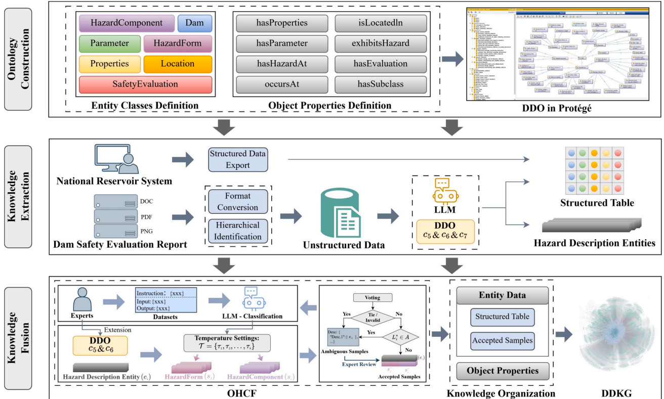
Fig. 1. Construction framework of DDKG.
