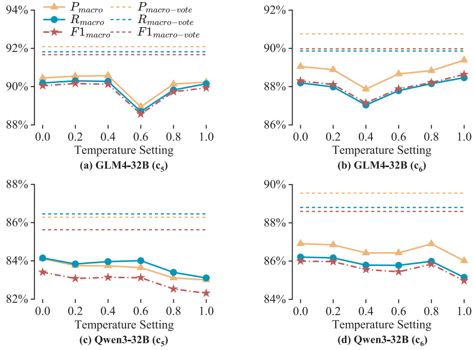
Fig. 7. Model performance under temperature perturbation and voting strategy.
