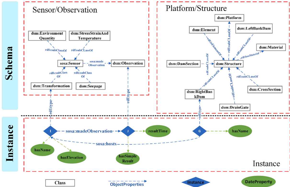
Fig. 6. Knowledge graph related to Sensor, Observation and Structure.
