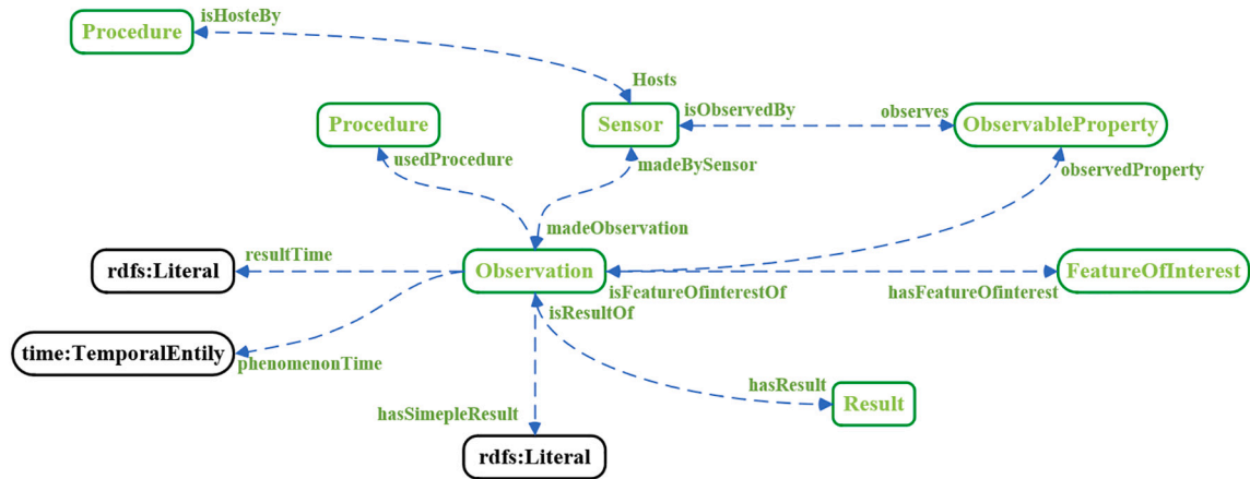
Fig. 2. Classes and relationships involved in Observation (SOSA).
