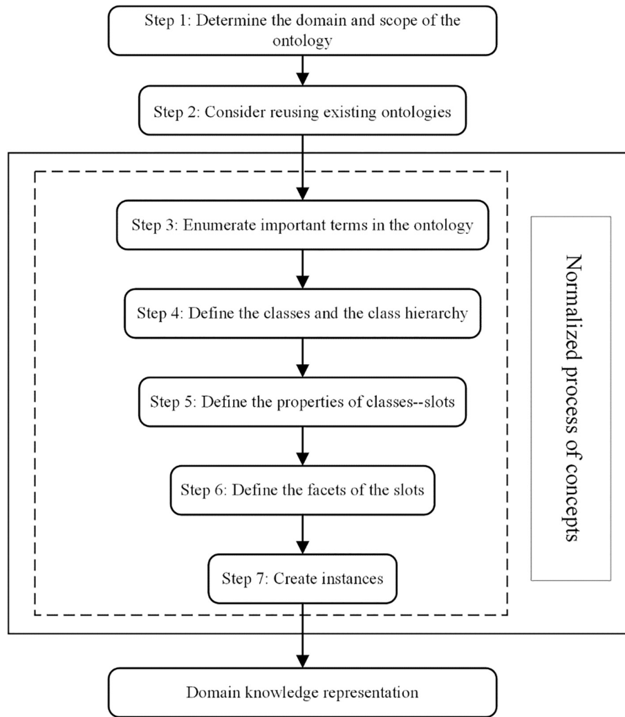
Fig. 1. Top-down modeling process using the Noy & McGuinness approach.
