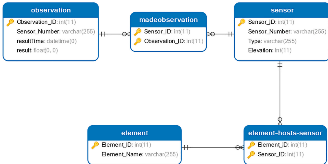
Fig. 8. Table structures in MySQL (partial view).
