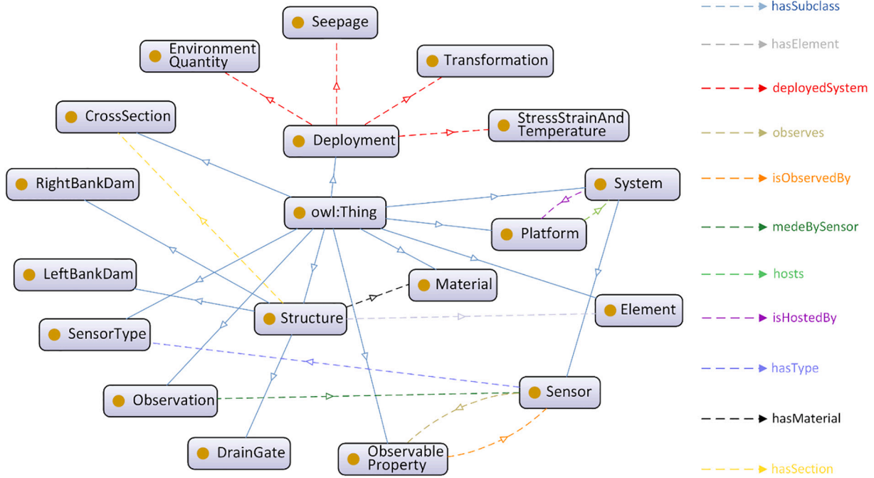
Fig. 5. Class hierarchy of OntoDSMS established in Protégé.
