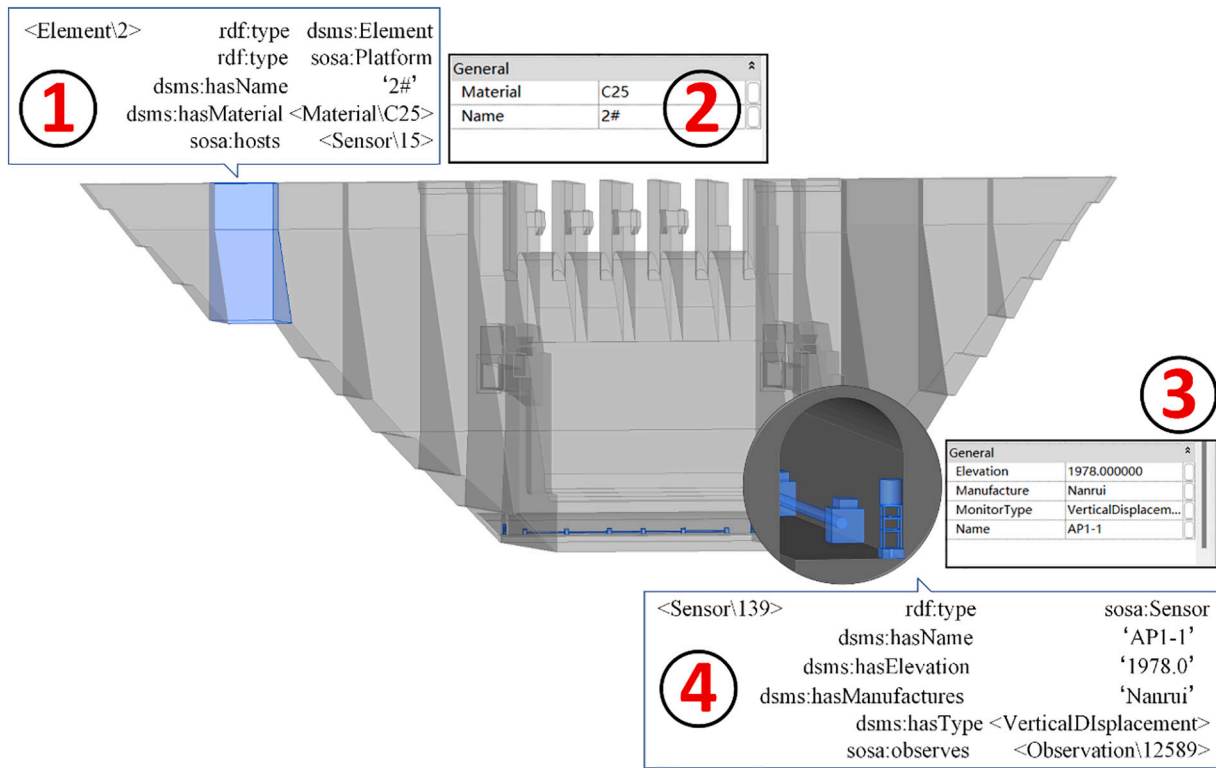
Fig. 7. Extracting context information from the BIM environment and the corresponding description in OWL.
