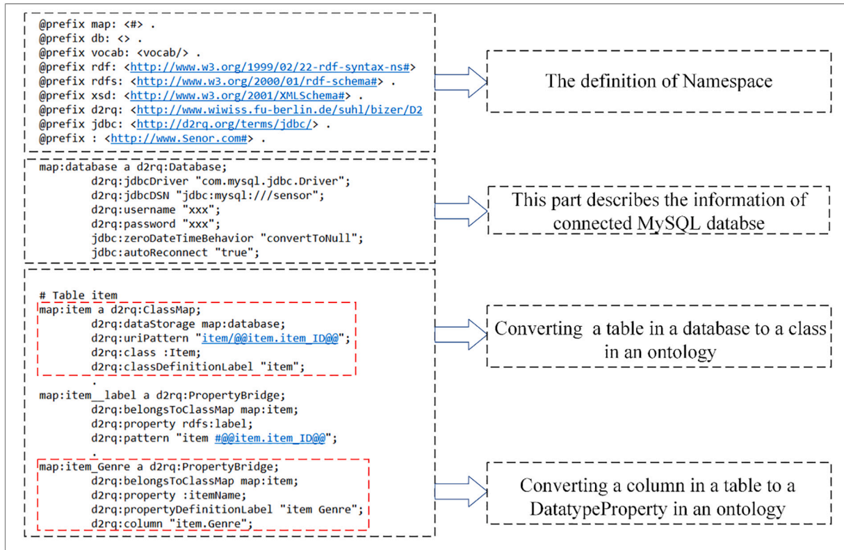
Fig. 3. Schema of the modified mapping file (partial view).
