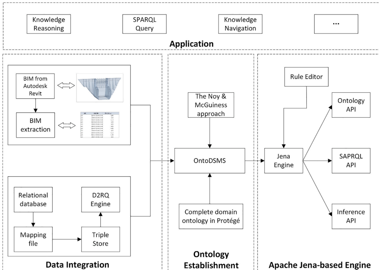
Fig. 4. Framework of managing monitoring information based on the OntoDSMS.
