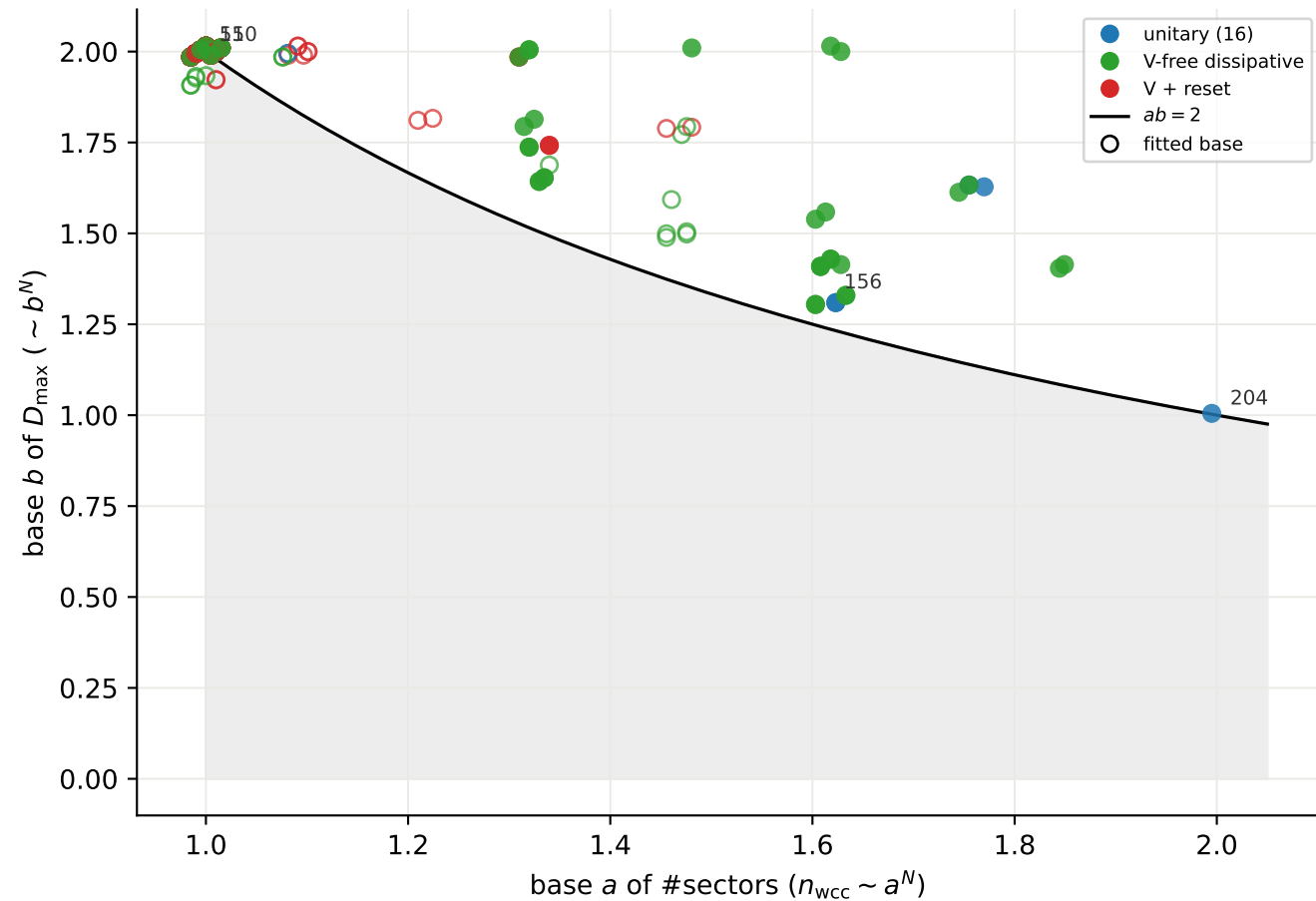
F1 sector map, 254 rules (obc0) — exact for BOTH experiments; 2 irregular omitted
