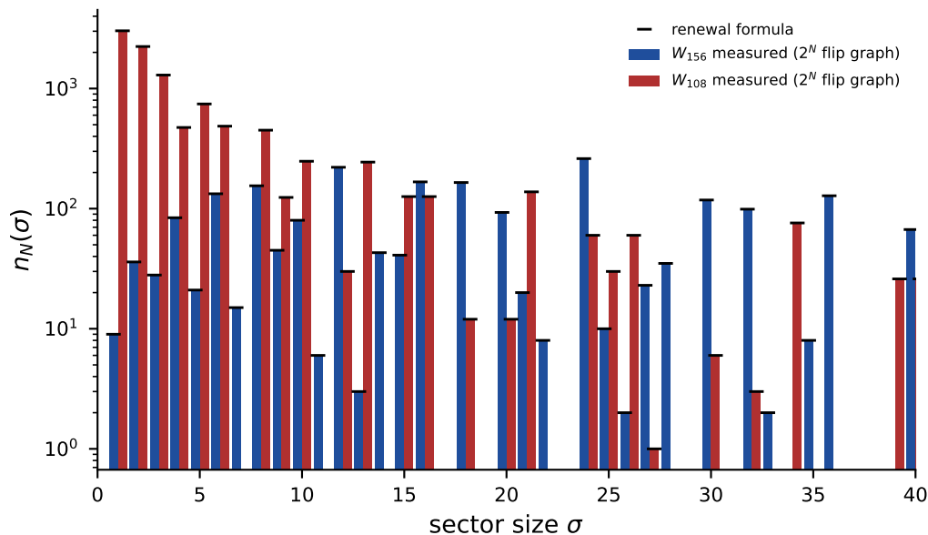
(a) obc0, N = 16 : the gaps in the W_{108} comb are the non-Fibonacci \sigma
