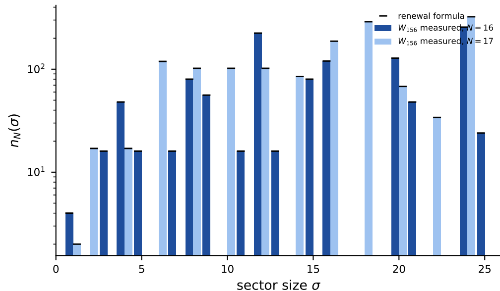
(b) pbc: consecutive N populate DISJOINT sizes ( N \equiv \text{sopfr} + \Omega )
