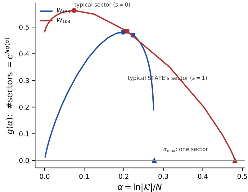
(b) the spectrum, g = \text{Legendre transform of } \ln \lambda_s
