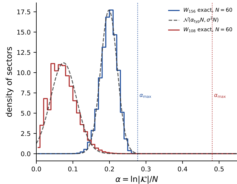
(a) the sizes are log-normal
