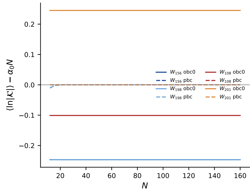
(c) the ring has no offset; the chain's is rule-dependent
