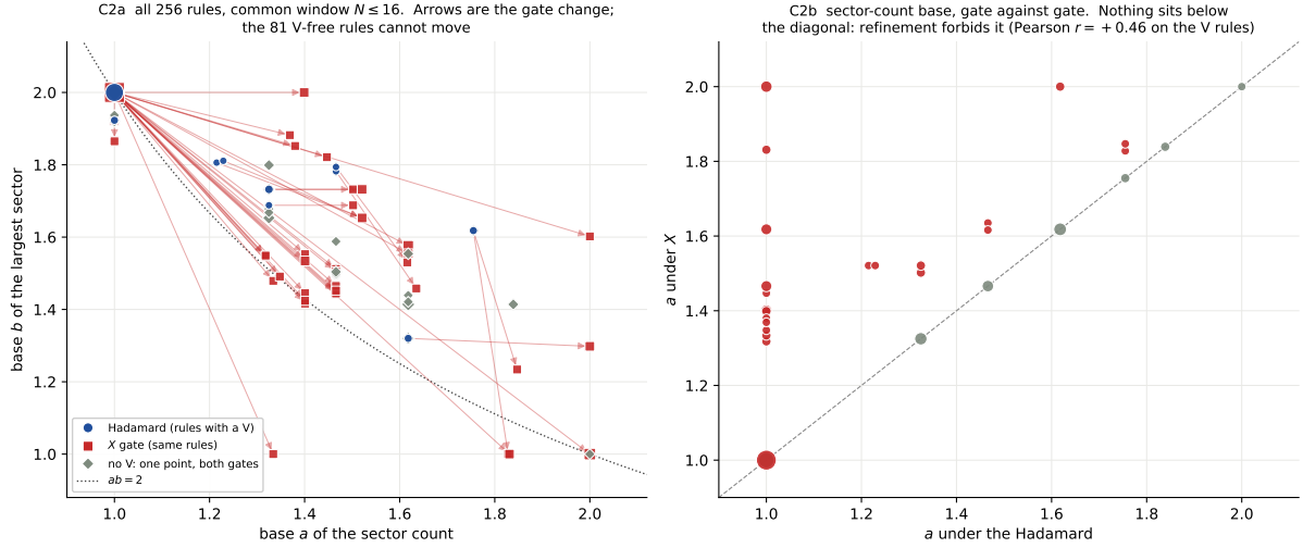
Figure 1: C2, all 256 rules on a common window. Left: the sector plane, Hadamard point (circle) joined to X point (square) for each rule that has a V; the 81 V-free rules are drawn as diamonds, one point each, because the gate cannot move them (Corollary 2). Almost every Hadamard point sits at (1, 2) — one giant sector — and the gate change fans them out to the right. Right: the sector-count base under one gate against the other. Nothing lies below the diagonal, which is Corollary 1 drawn.
