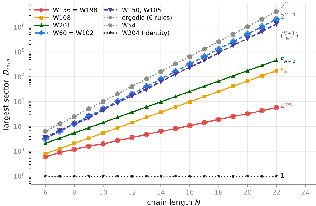
Largest sector vs system size, all unitary rules (obc0)
