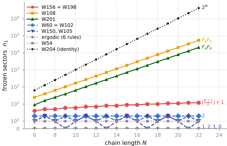
Frozen states vs system size (obc0)
