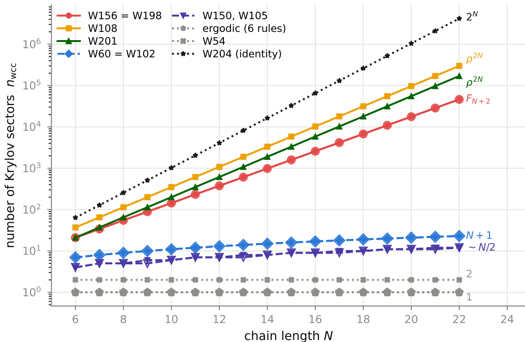
Sector count vs system size, all unitary rules (obc0)
