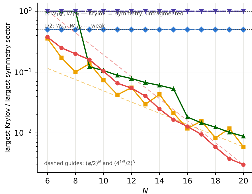
(b) the criterion: D_{\max}(s^*)/\dim s^*
