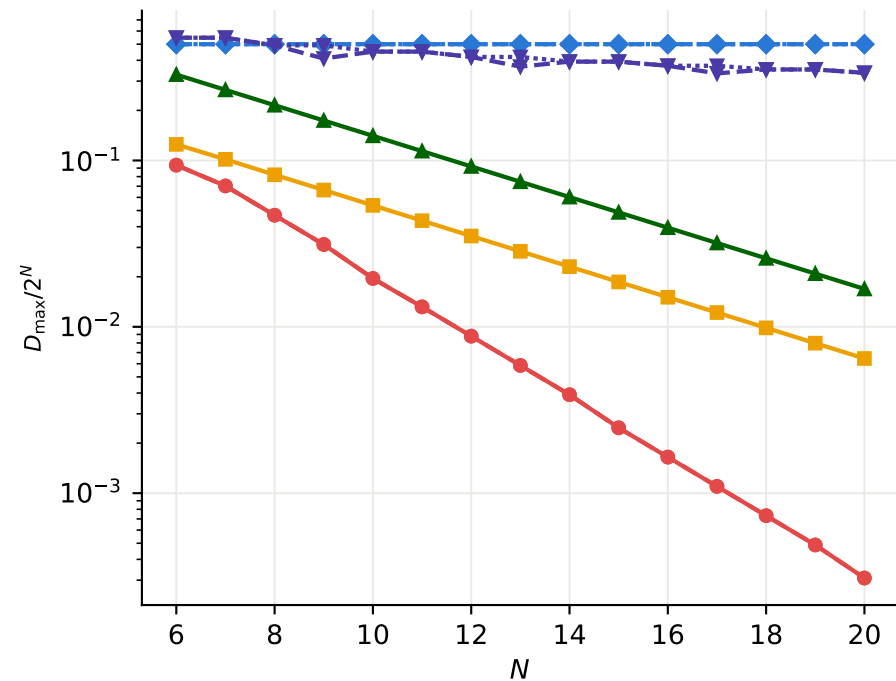
(a) the crude ratio D_{\max}/2^N
