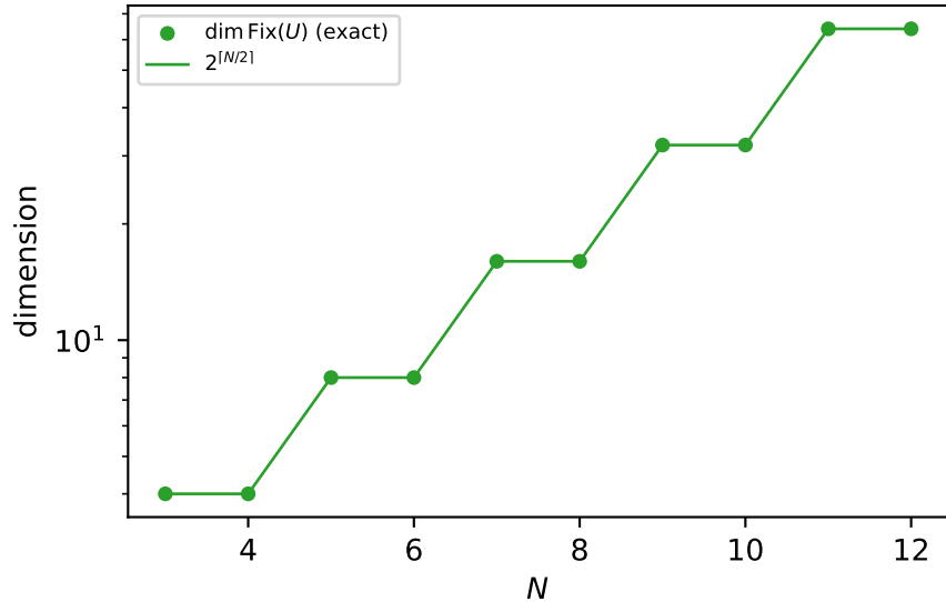
stationary states: dark superpositions inside sectors
