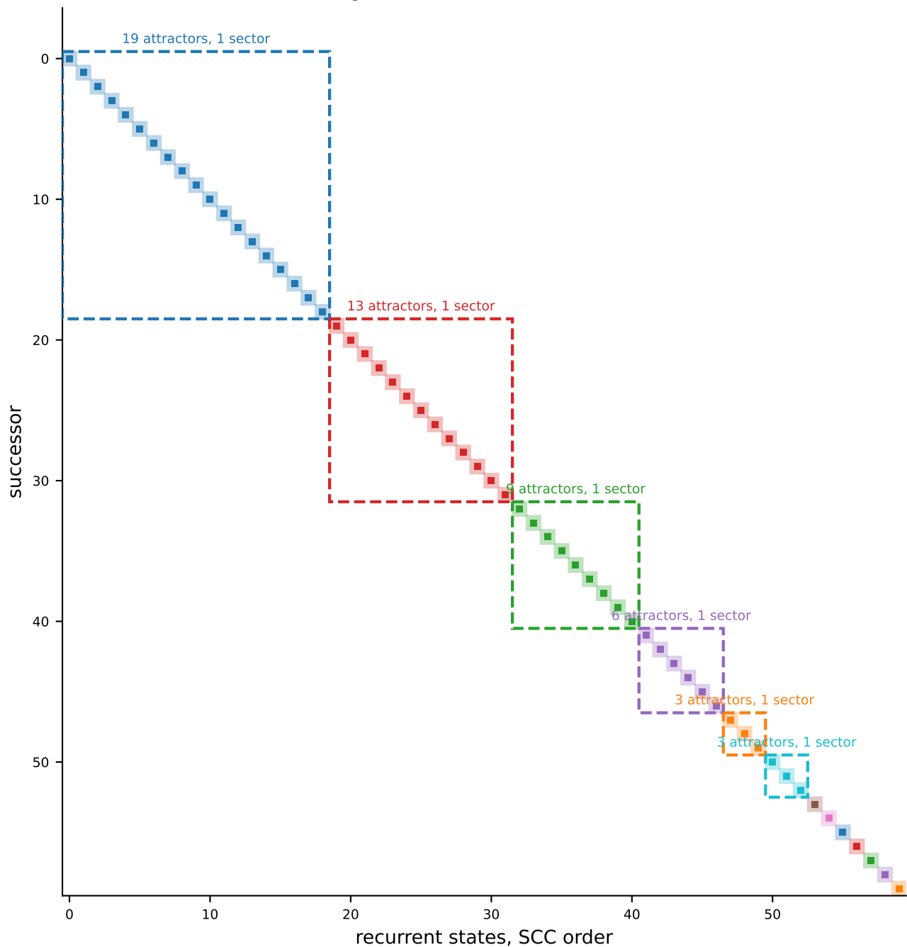
W100 (IDIV), obc0, N = 10 : the recurrent corner 60 terminal SCCs holding 60 states, in 13 sectors (6 of them multi-attractor)
