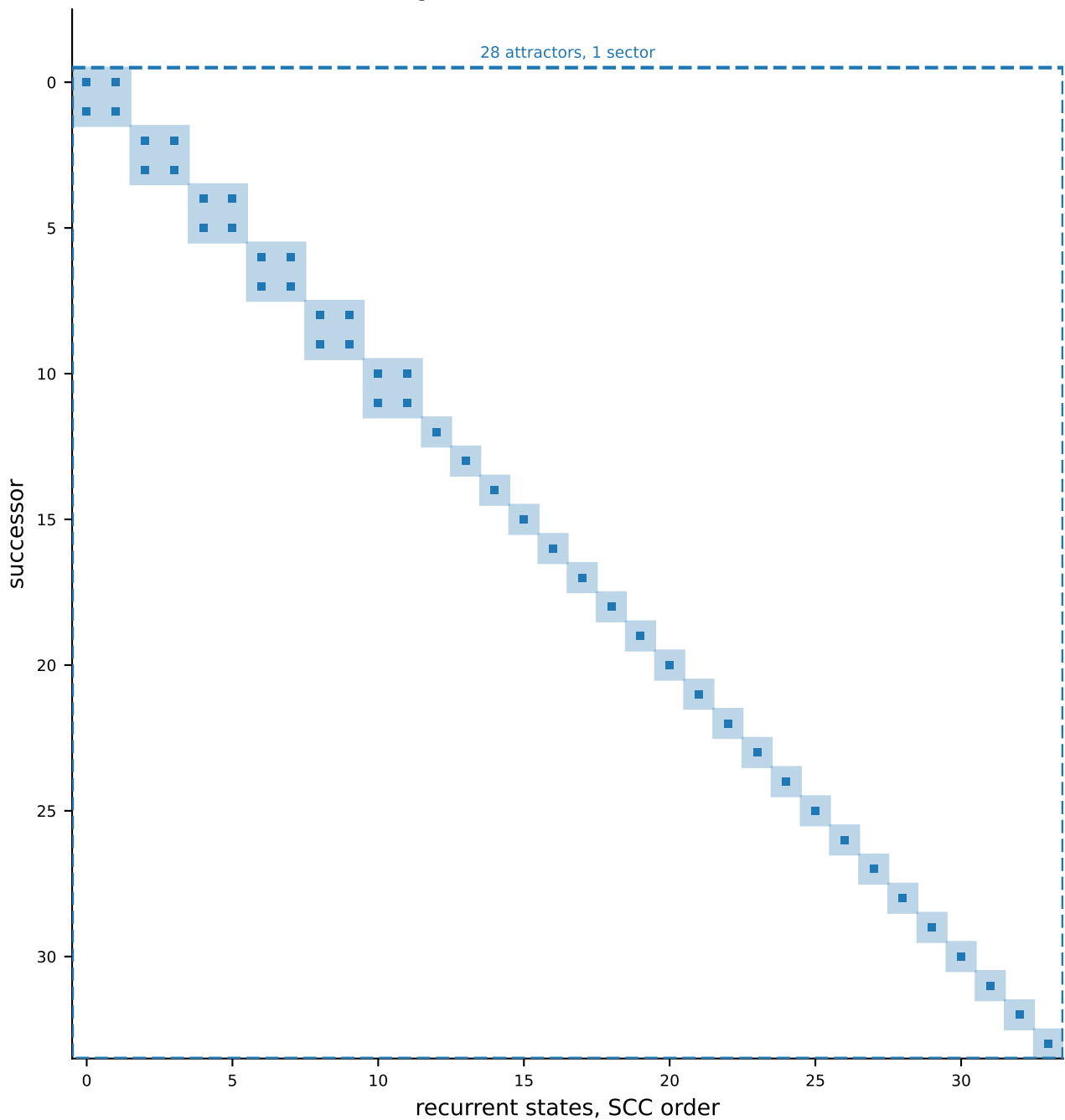
W203 (VEII), obc0, N = 10 : the recurrent corner 28 terminal SCCs holding 34 states, in 1 sectors (1 of them multi-attractor)
