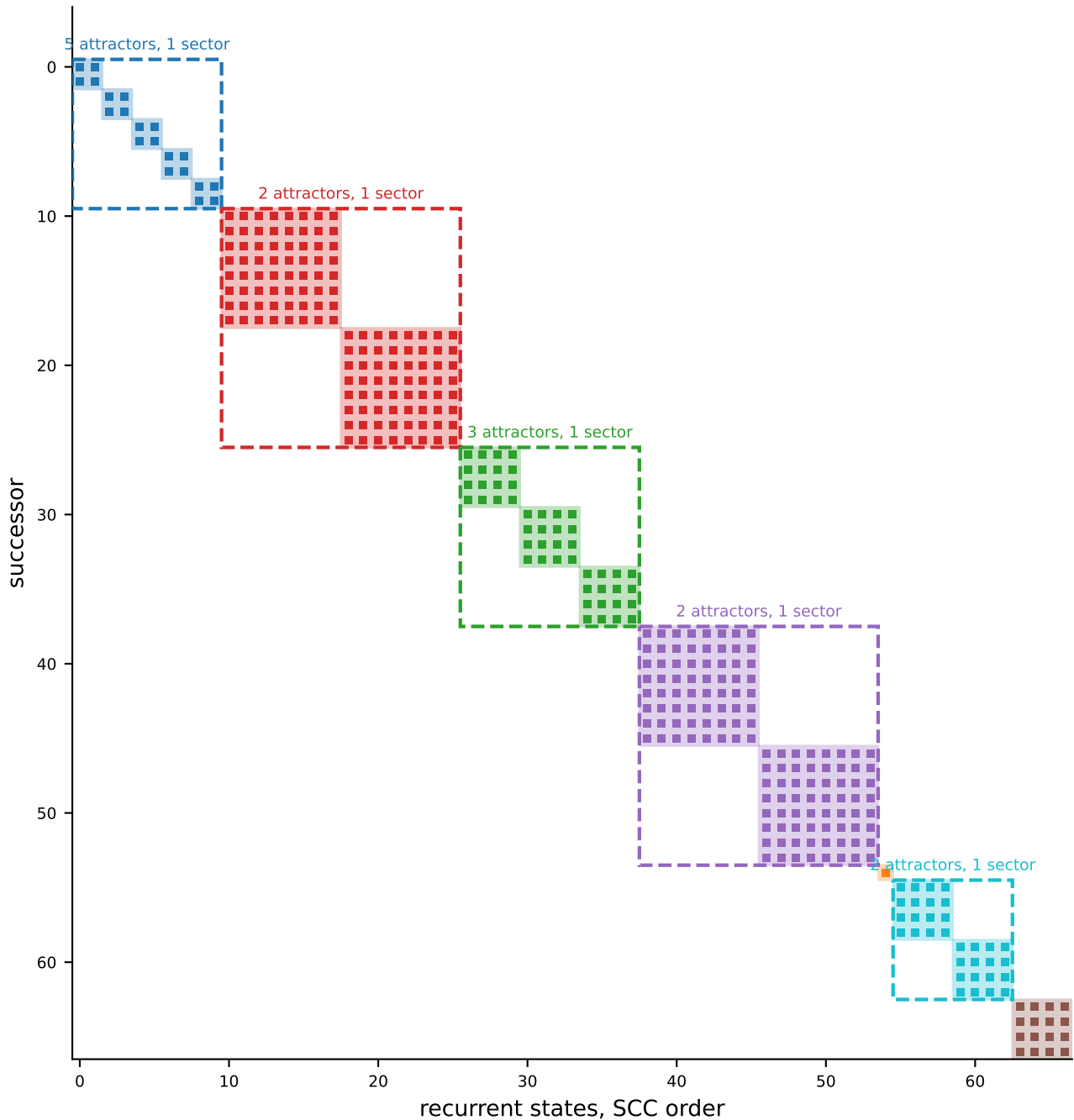
W29 (EIVD), obc0, N = 10 : the recurrent corner 16 terminal SCCs holding 67 states, in 7 sectors (5 of them multi-attractor)
