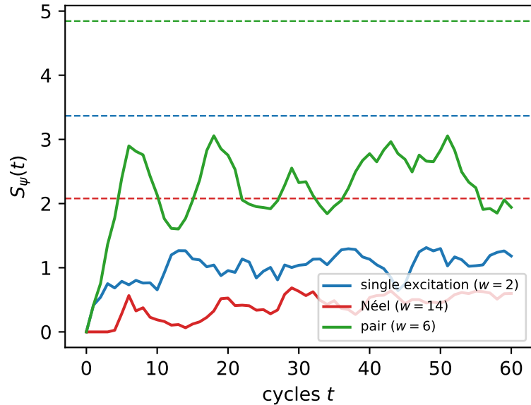
N = 14 ; dashed = kinematic ceiling
