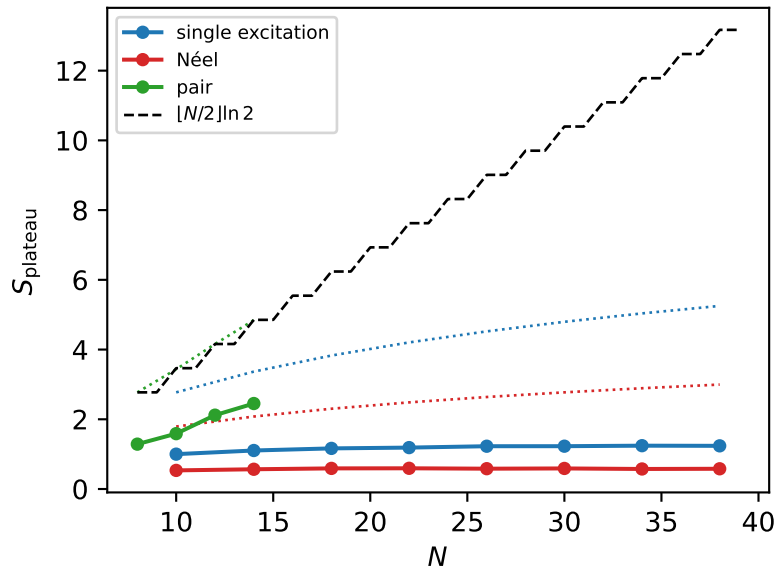
area law vs volume law (dotted = ceiling)
