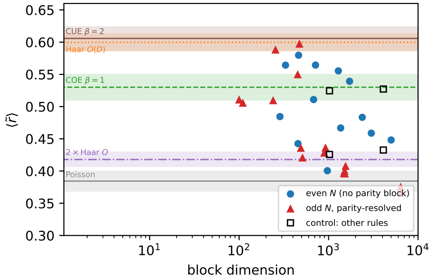
spacing-ratio statistic against generated references
