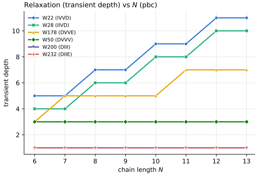
Figure 4: Transient depth vs. N (pbc) for selected dissipative rules.
