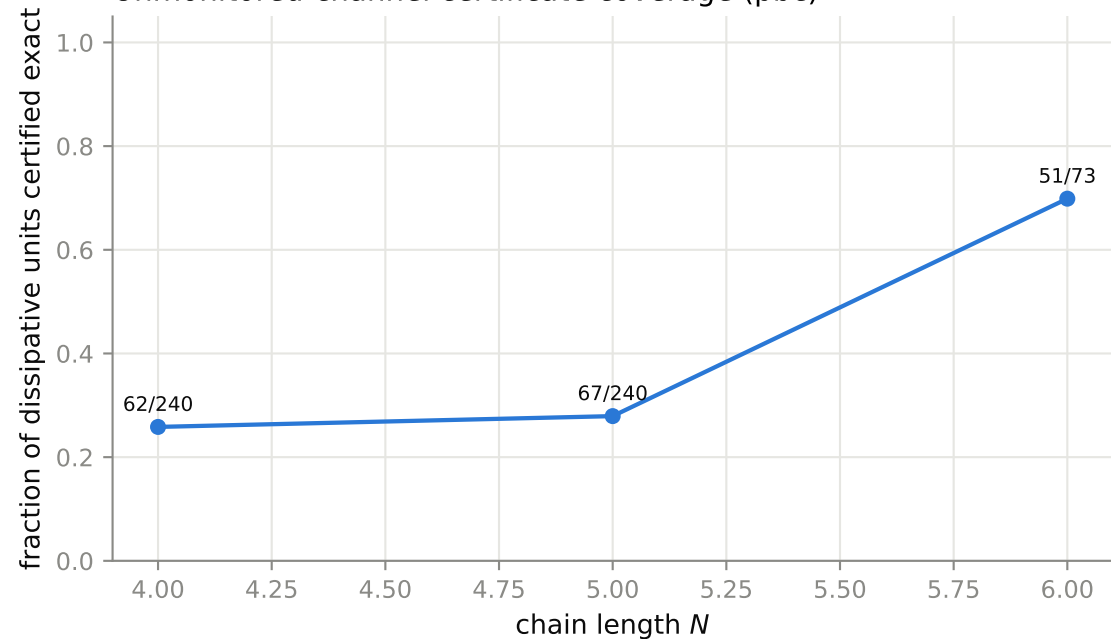
Unmonitored-channel certificate coverage (pbc)
