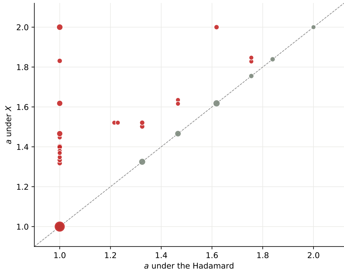
C2b sector-count base, gate against gate. Nothing sits below the diagonal: refinement forbids it (Pearson r = +0.46 on the V rules)
