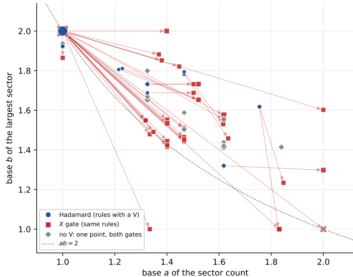
C2a all 256 rules, common window N \leq 16 . Arrows are the gate change; the 81 V-free rules cannot move
