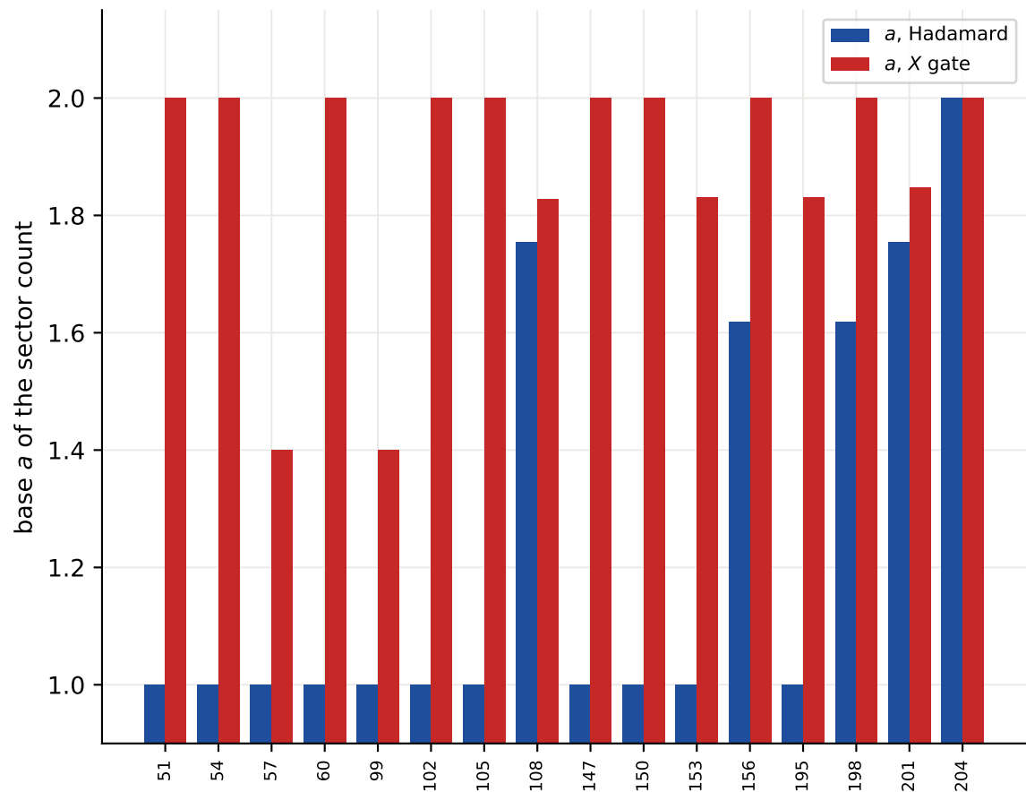
C1b the sector-count base, rule by rule. 204 is the only rule the gate does not move
