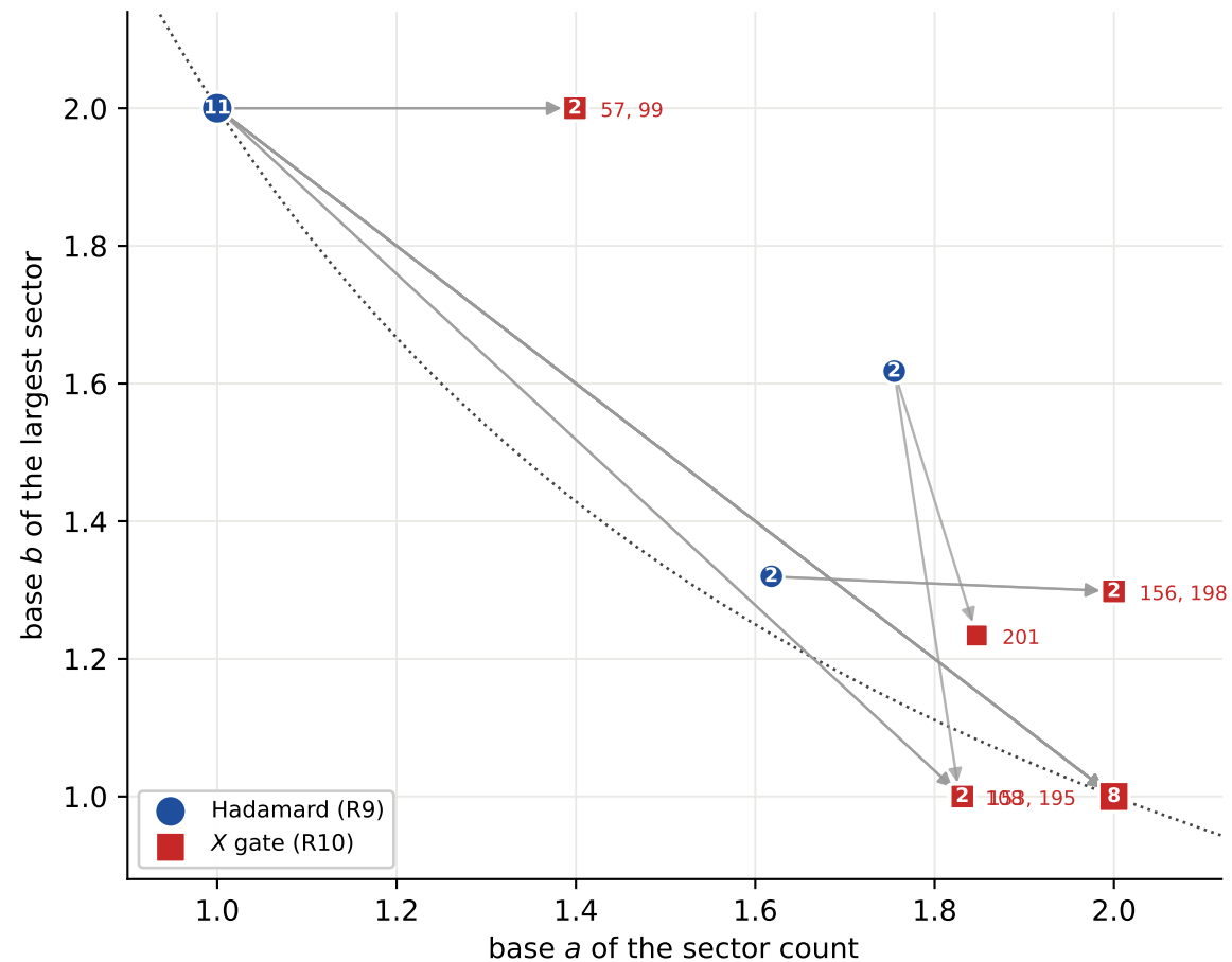
C1a the 16 rules that are unitary under H and reversible under X : same table, different gate
