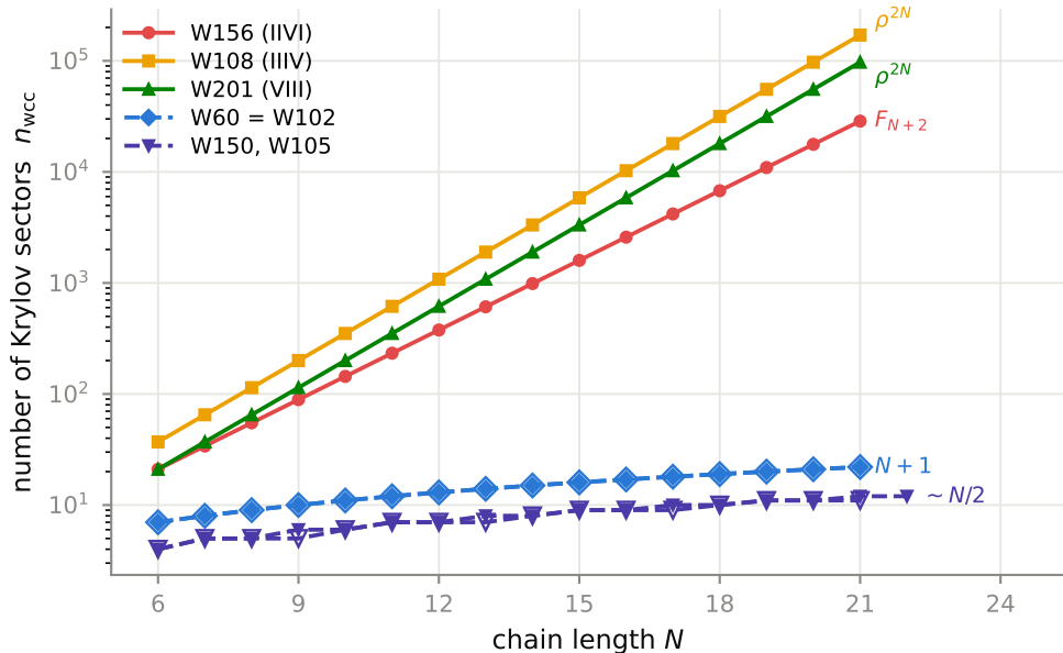
Sector count vs system size (obc0)
