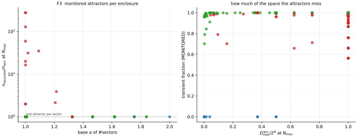
Figure 3: F3, monitored structure inside one enclosure . Left: n_{\text{recurrent}}/n_{\text{wcc}} at the largest N reached, against the sector base. Right: the monitored transient fraction against D_{\text{max}}^{\text{wcc}}/2^N . The attractor counts are monitored; the sector quantities are not.
