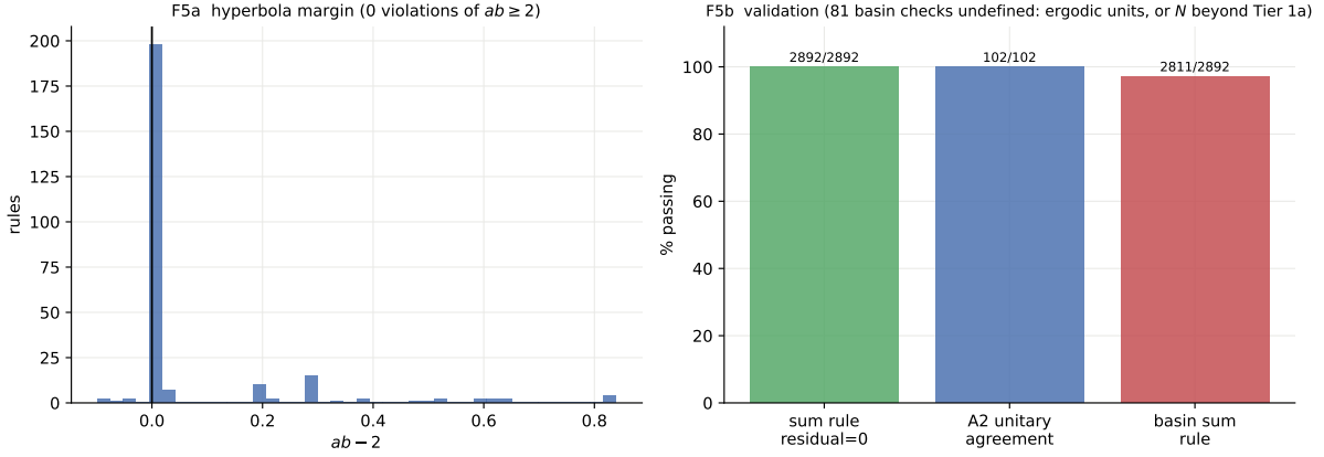
Figure 5: F5, validation panel. Left: distribution of the hyperbola margin ab - 2 . Right: pass rates for the sum rule A1 (residual identically zero), the unitary agreement A2, and the monitored basin sum rule.
