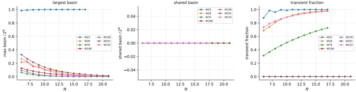
Figure 4: F4, basin structure (MONITORED) . Largest basin, shared basin and transient fraction against N for selected rules. Two things to read off. The shared basin is identically zero for every rule shown: each transient state funnels to a unique terminal SCC, so the basins alone already partition the transient part and no state is ambiguous between attractors. And the two unitary rules (156, 201) sit at transient fraction 0 by construction — every state is recurrent — which is the cleanest illustration of why the transient fraction is a monitored quantity and not a sector one. Tier 1d’s certificate T3 gives certified zeros for the unmonitored basins of the V-free rules, so for those 80 rules the monitored and channel populations coincide and these curves are channel-exact; for the rest they are monitored-only.
