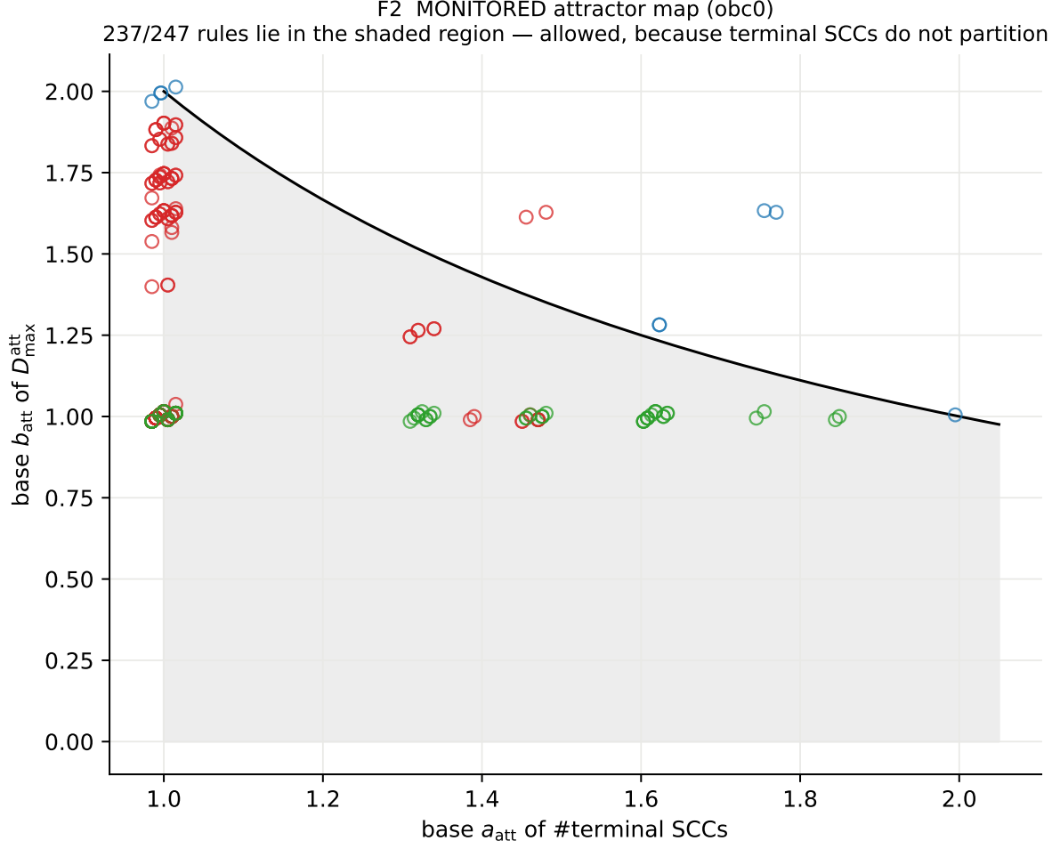
Figure 2: F2, monitored attractor map (MONITORED only) . The same plane for terminal SCCs. The hyperbola is drawn only as a reference and the region below it is shaded to make the contrast with Fig. 1 explicit: rules may and do sit there, because terminal SCCs do not partition the basis. The deficit 2 - a_{\text{att}}b_{\text{att}} is an observable, not a failure.
