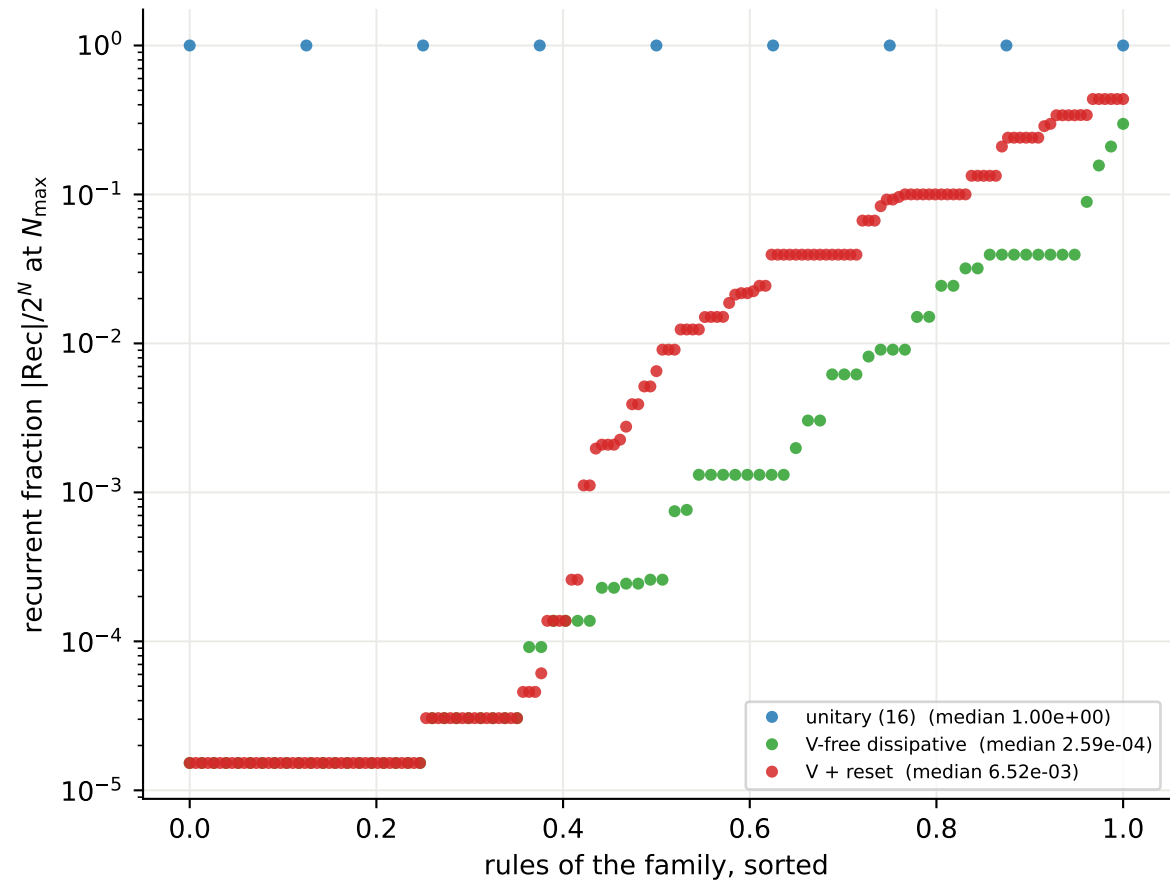
F9b the same, unfitted: the share of the basis that is recurrent at the largest N computed
