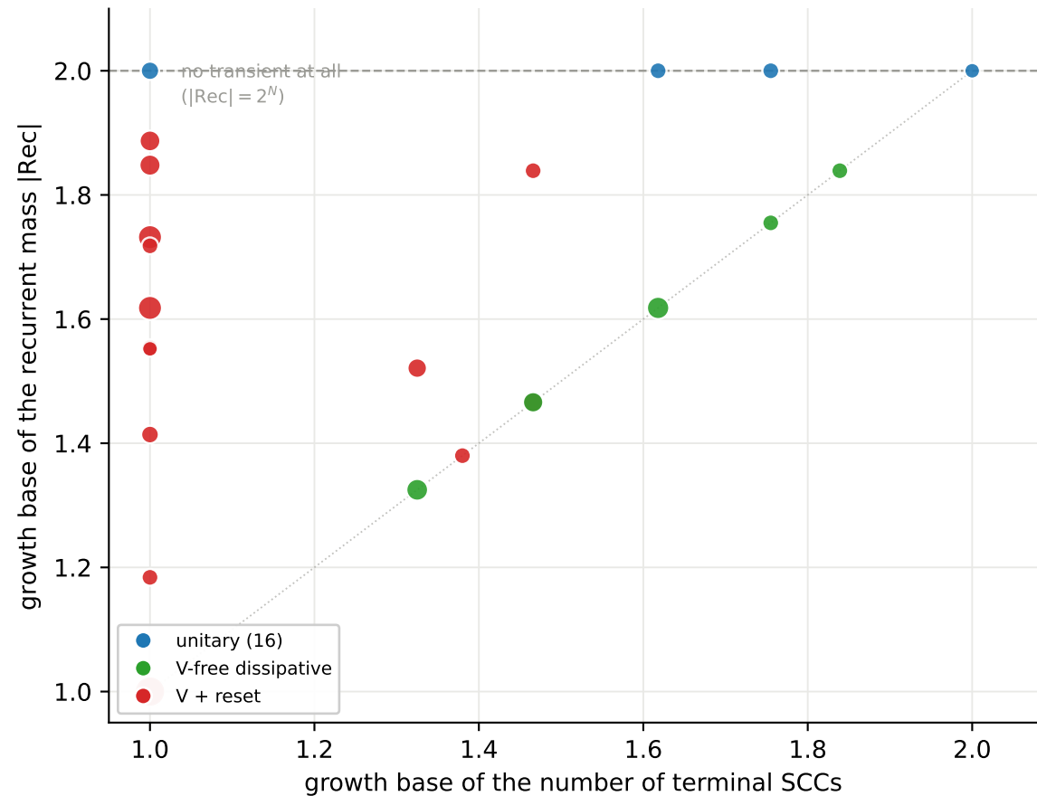
F9a terminal SCCs against transient states: how much of the basis survives to late times
