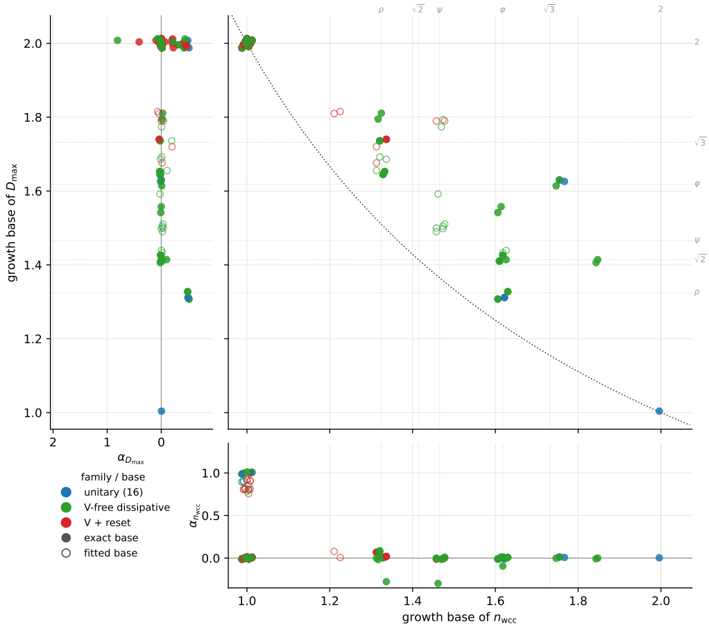
Figure 4: F8, the sector map in corner form (obc0). Main panel: the map of Figure 1 with the exclusion curve. Bottom margin: the sector count's sub-leading power against its base — the column at a = 1 splits into \alpha \simeq 0 (genuinely one sector) and \alpha \simeq 1 (the pinned-frontier rules of §9.5, a linear number of them), which the main panel cannot distinguish. Left margin: the D_{\max} power, where the binomial family's -\frac{1}{2} is visible at b = 2 . Filled marker = exact base.
