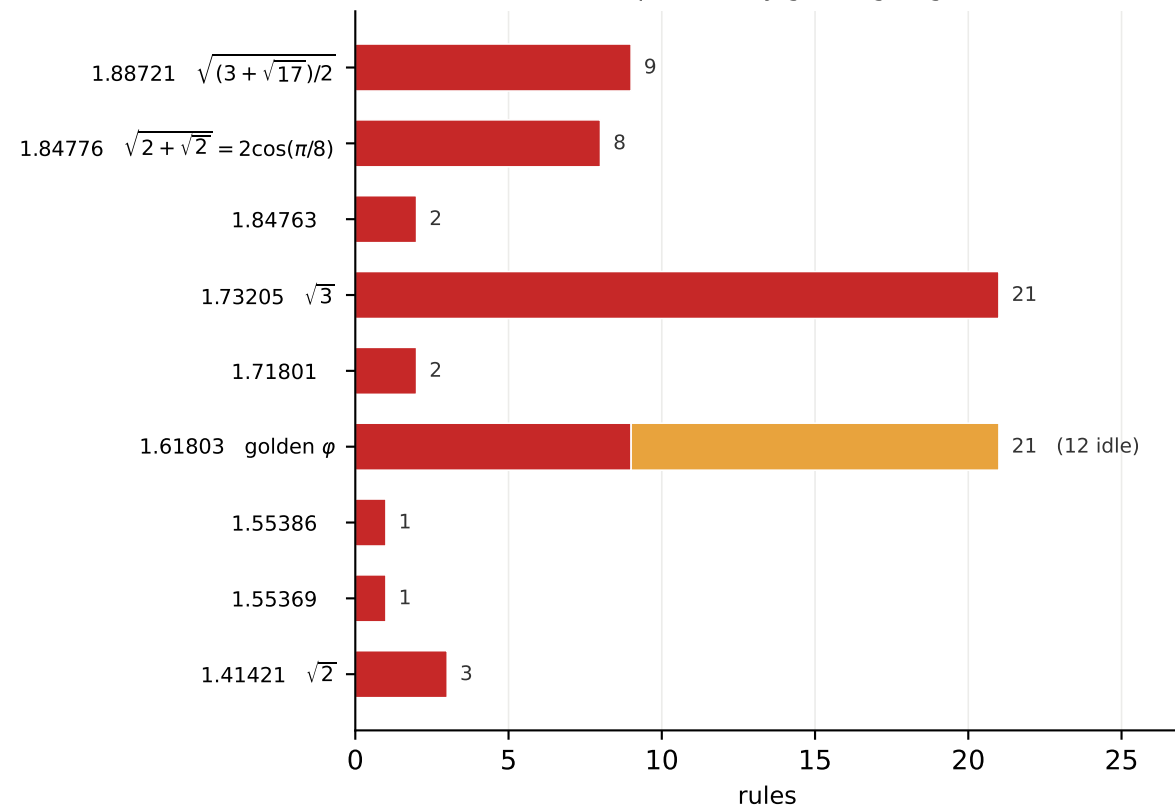
the tower: 68 V+reset rules with a flat attractor count and an exponentially growing largest attractor
