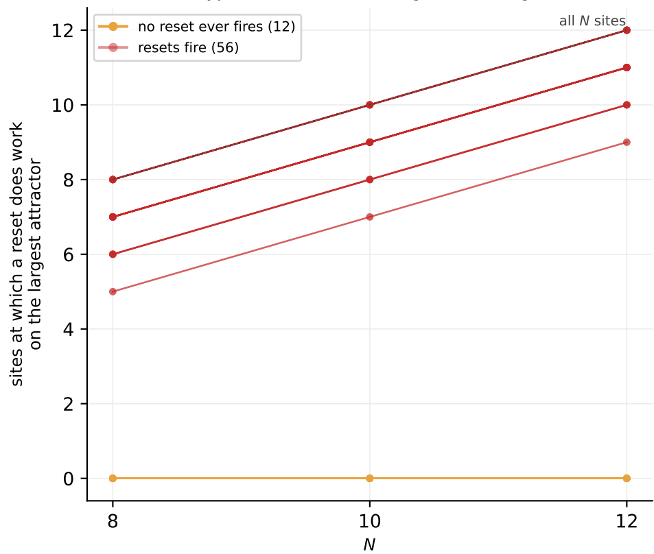
the hypothesis, tested: idle (gold) vs firing (red)
