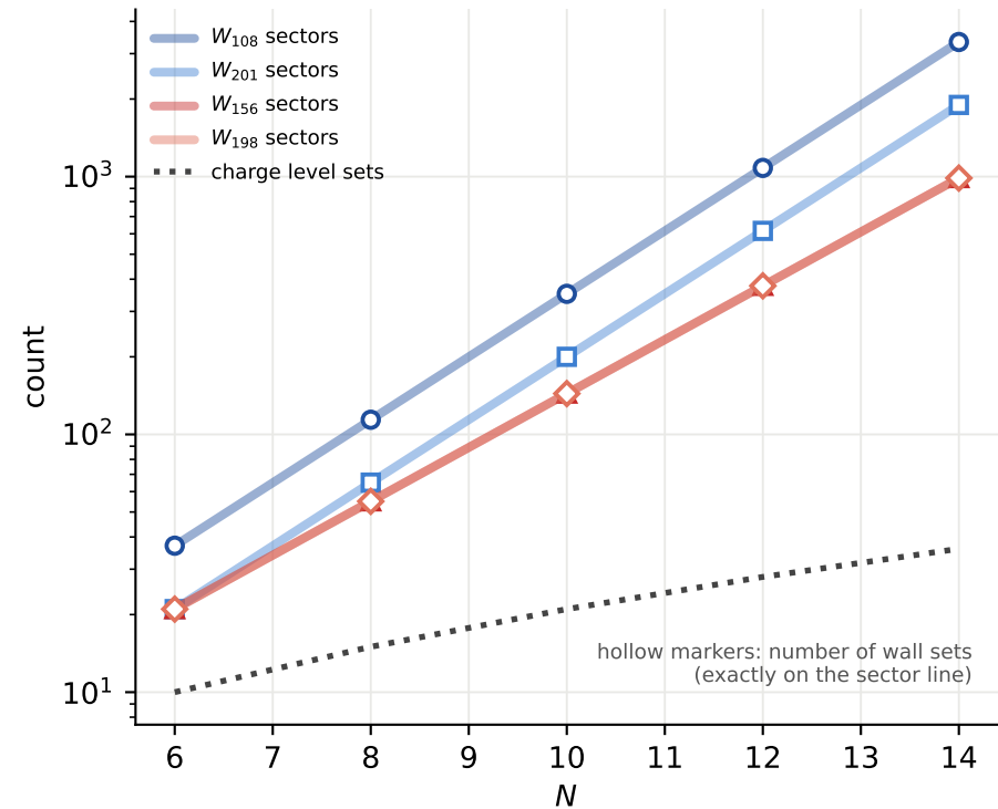
(a) walls track the sectors; charges do not
