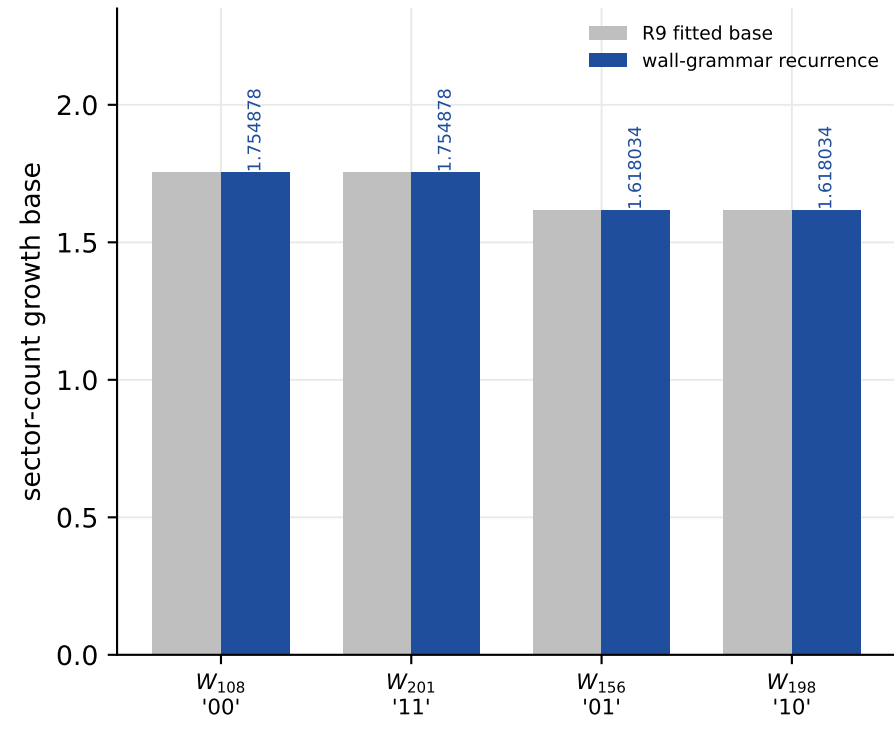
(c) the exponent comes out of the grammar
