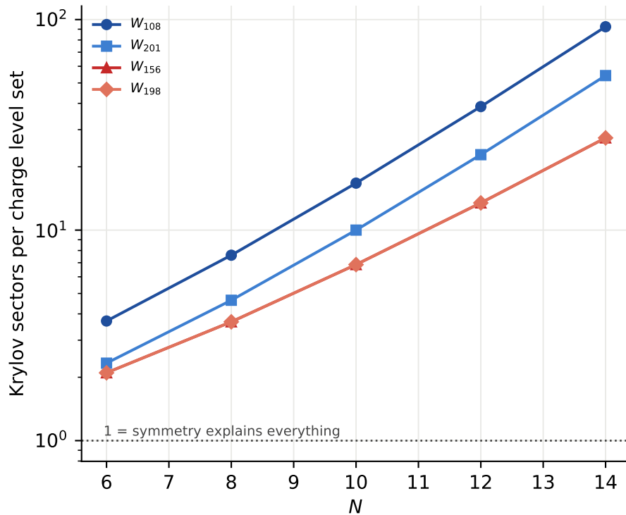
(b) beyond the symmetry: level sets of |W_{\text{even}}| , |W_{\text{odd}}|
