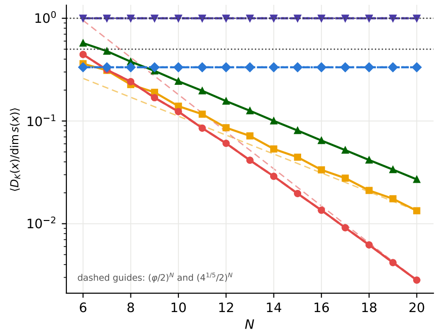
(c) fraction of its symmetry sector a random state reaches
