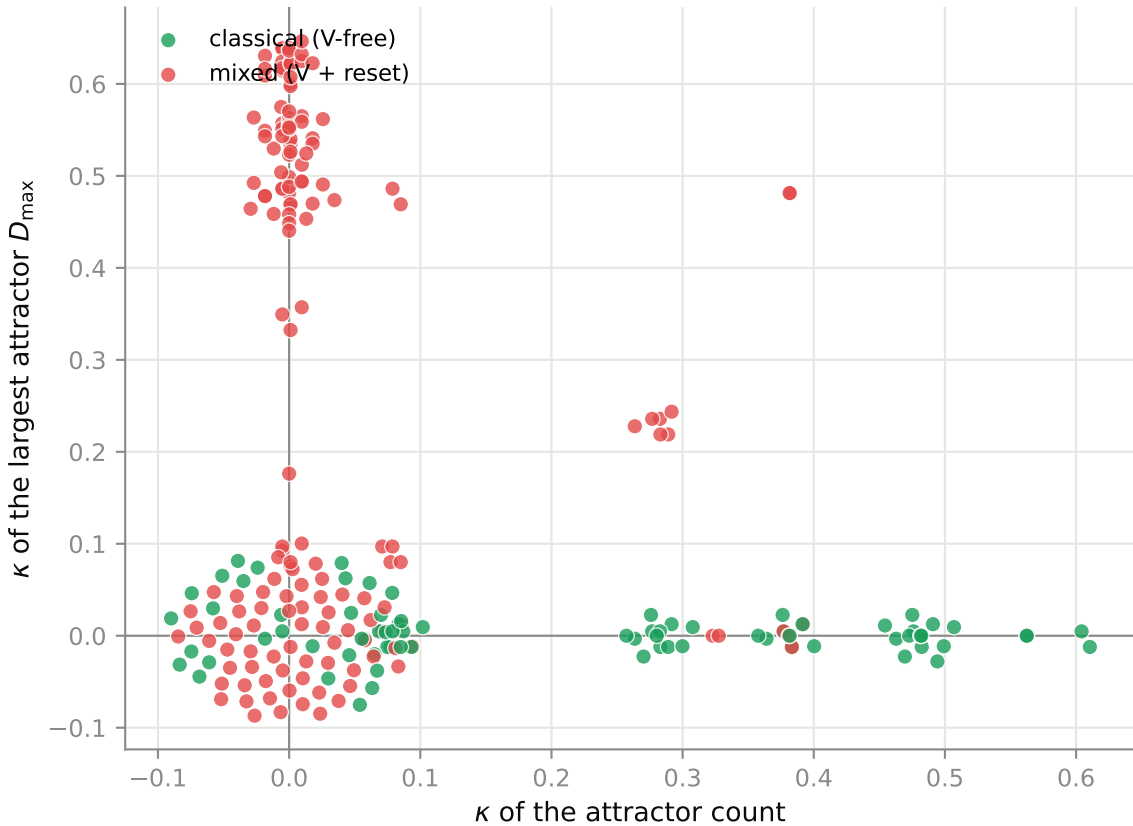
Dissipative growth-rate map (obc0, 238 rules)
