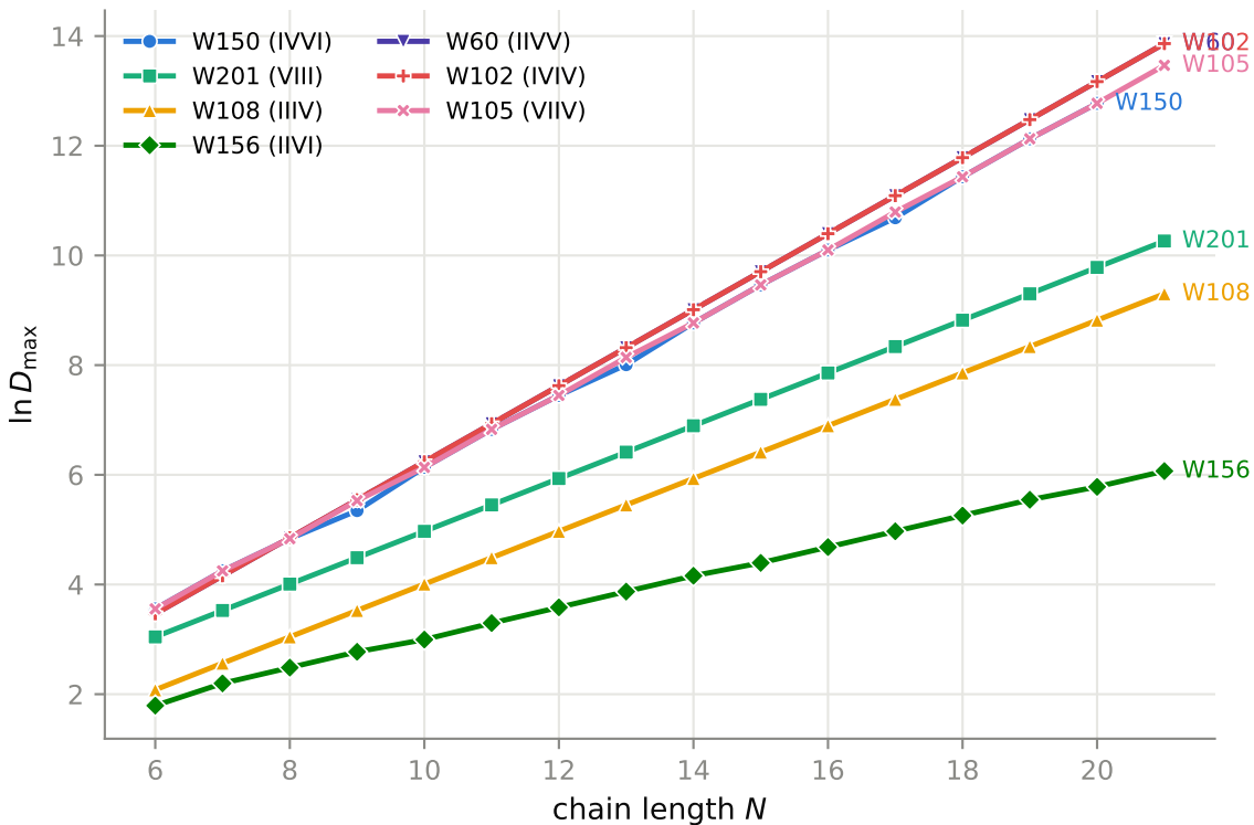
Largest sector vs system size (obc0)
