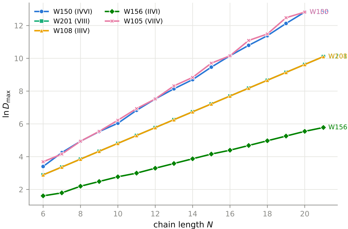
Largest sector vs system size (pbc)
