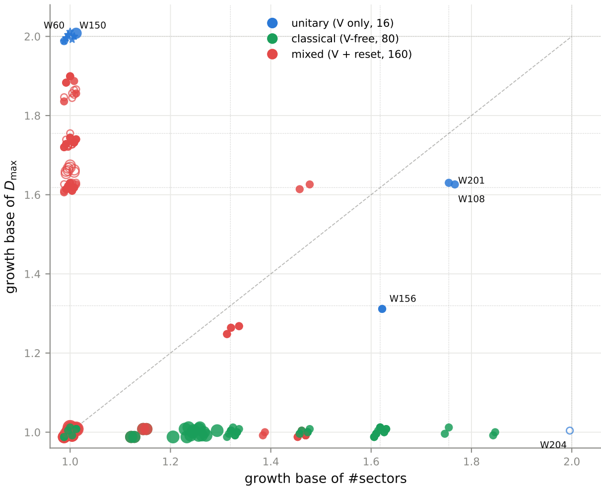
Growth-base map (pbc): colour = family, size \propto poly. degree
