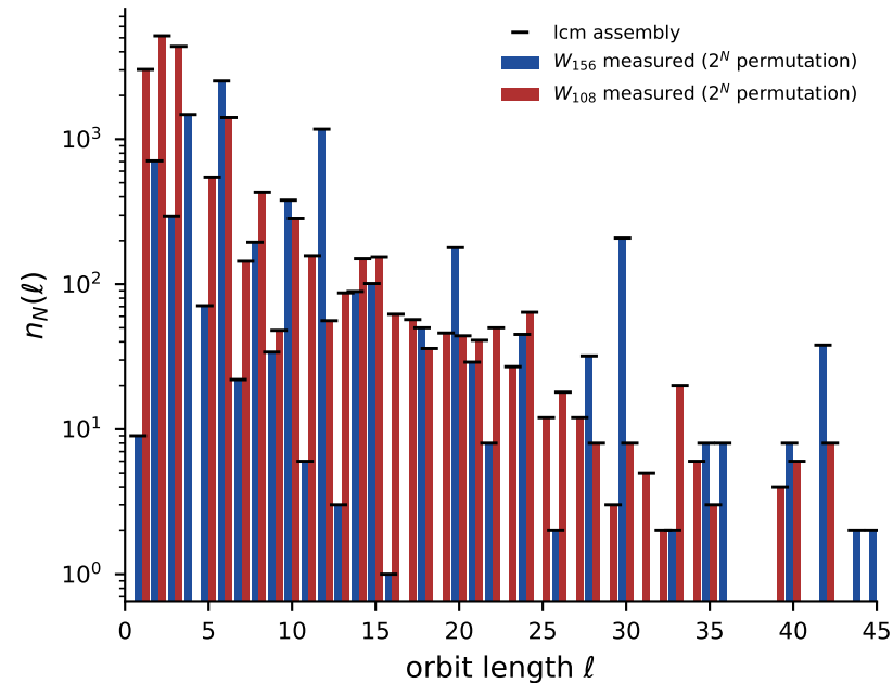
(a) orbit lengths, obc0, N = 16
