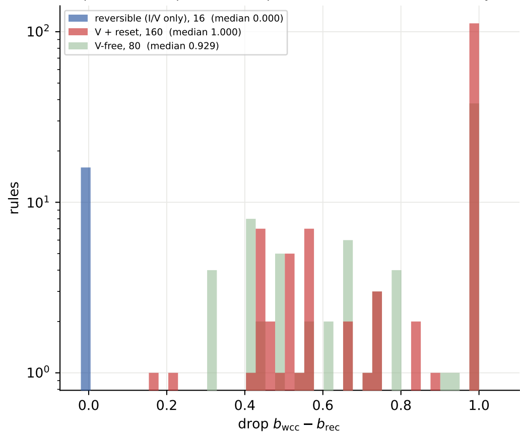
X4b how far the rule falls. zero drop = the whole sector is periodic; a drop of 1 = an exponential sector with a bounded cycle
