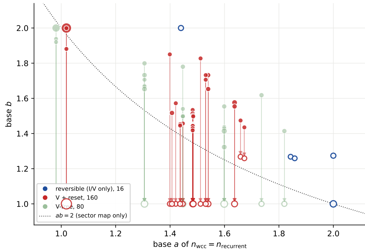
X4a filled marker: largest sector. hollow: longest cycle. every move is straight down, because a is shared by (F1)
