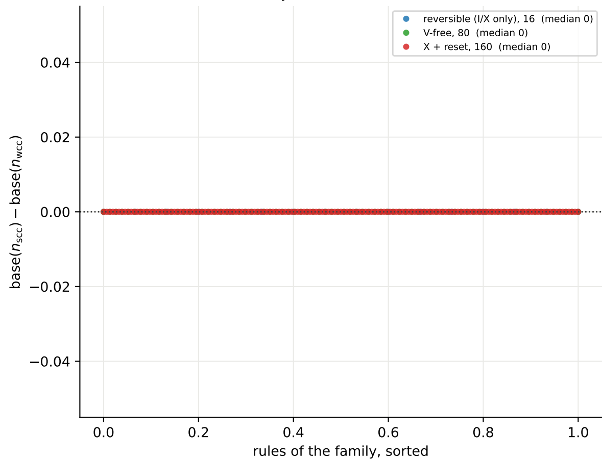
X9b the same as a per-rule ratio, each family sorted: how many attractors a sector carries
